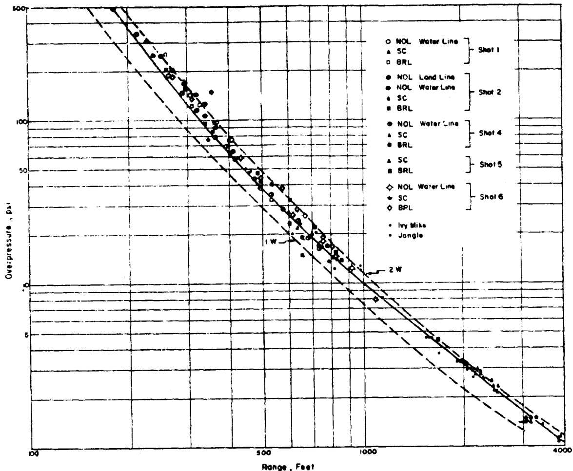
Figure 2.4 Composite overpressure versus scaled ground range, Shots 1 through 6.
