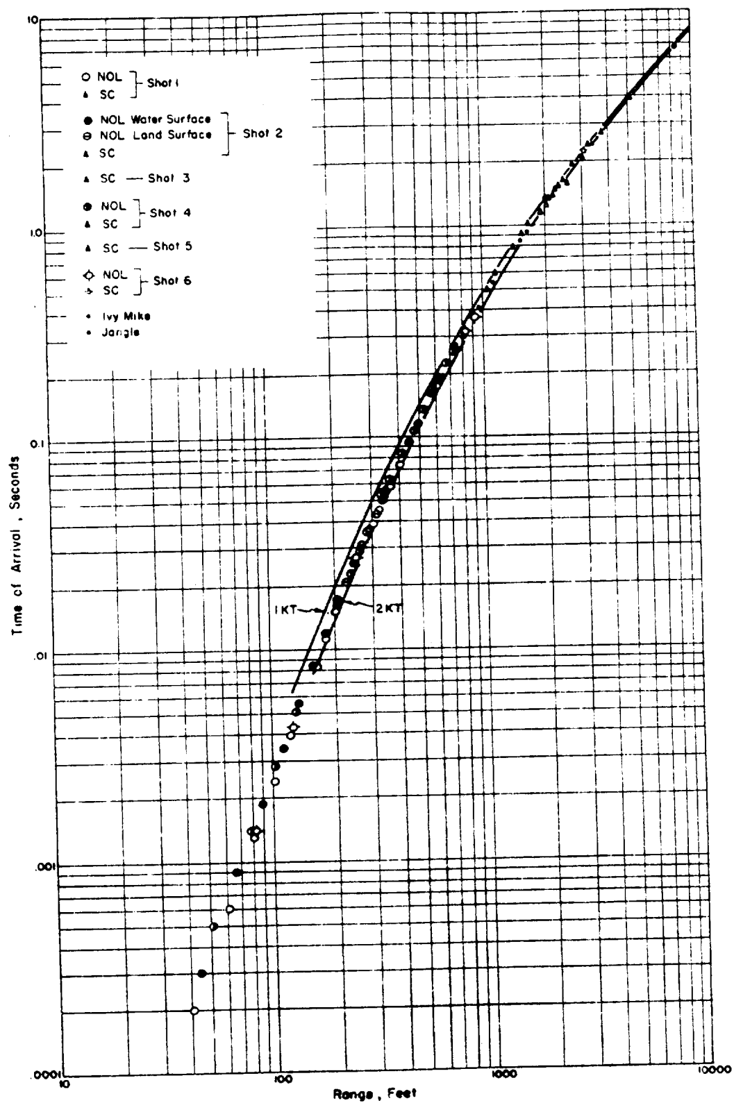
Figure 2.5 Composite scaled time of arrival versus scaled ground range, Shots 1 through 6.
