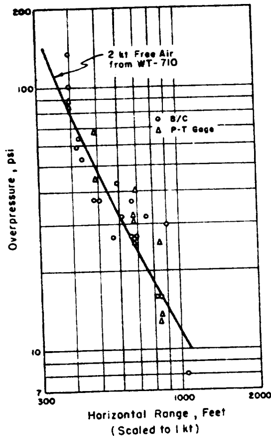
Figure 2.11 Averaged pressure-distance data.
