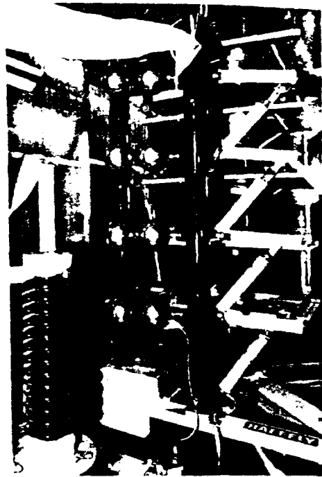
Part of an impulse generator used to study the properties of dielectric gases under steep voltage pulses such as would be encountered in the new pulsed power technologies being developed for fusion energy, particle beam weapons, and other applications.
