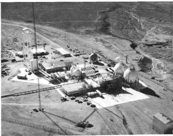
Test Cell C in 1967. Movable shields on test stand, right center, surround reactors during test. Building, lower right, can be moved on rails over reactors for weather protection.
