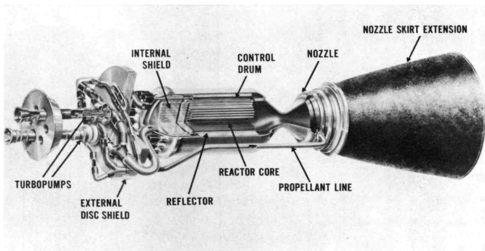
Drawing of the complete NERVA engine.
