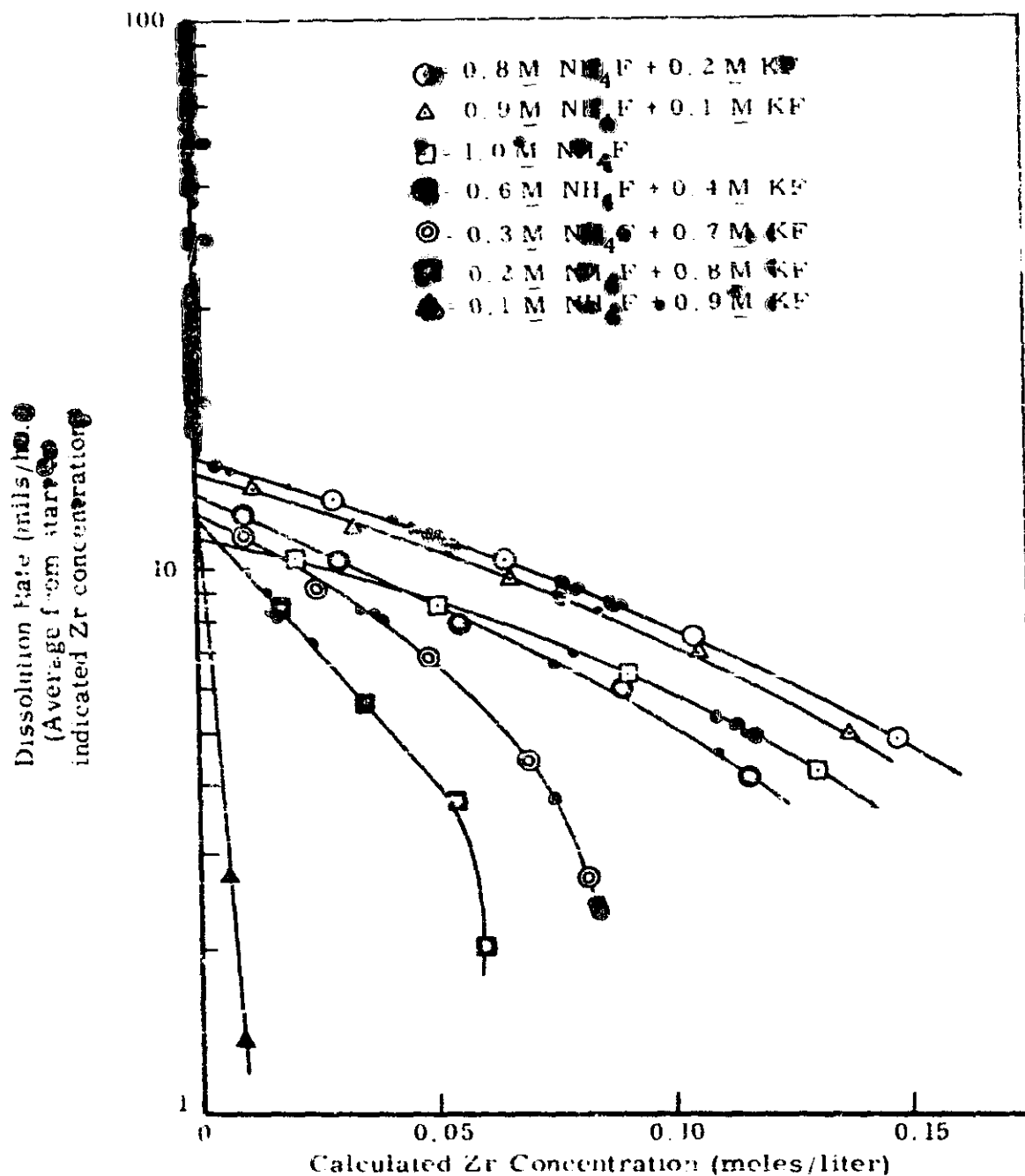
FIGURE 1 RATE OF DISSOLUTION OF ZIRCALLOY-2 IN \text{NH}_4\text{F} - \text{KF} MIXTURES
