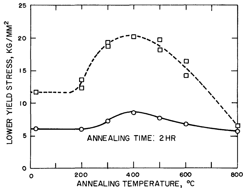
Fig. III-16 Effect of annealing on the lower yield strength of irradiated niobium. 69 \square , fluence = 2 \times 10^{18} neutrons/cm 2 ( E > 1 Mev); \circ , unirradiated.
