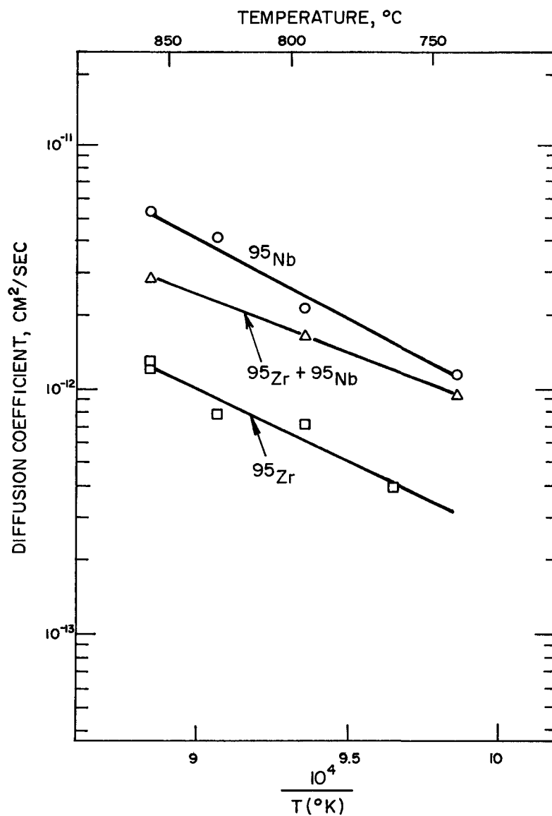
Fig. III-25 Temperature dependence of diffusion of 95 Zr, 95 Zr + 95 Nb, and 95 Nb in hcp zirconium. 124
