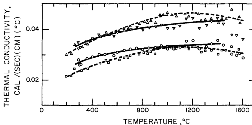
Fig. I-7 Calculated thermal conductivity of (U_{0.20}Pu_{0.80})N samples. 35a Metal-hydride (UPu)N : □, 86% theoretical density; Δ, corrected to 100% theoretical density. Carbothermic (UPu)N : ○, 89% theoretical density; ▽, corrected to 100% theoretical density.
