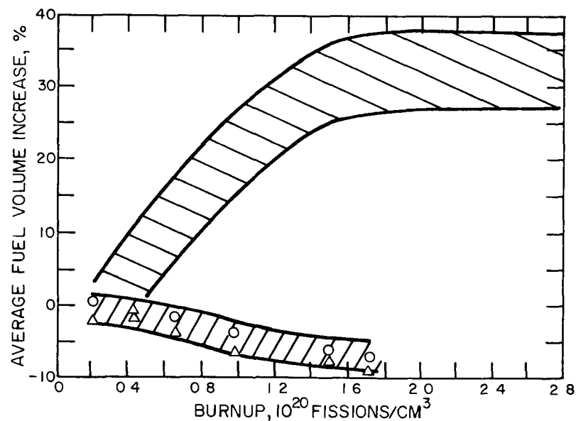
Fig. I-9 Effect of burnup on volumetric swelling of W-UO 2 cermet. 54 ZZZ , W-30 vol. % UO 2 , 20-mil cladding; o , W-42 vol. % UO 2 , 28% porosity, 40-mil cladding, vented; Δ , W-42 vol. % UO 2 , 28% porosity, 40-mil cladding.
