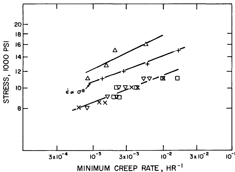
Fig. III-23 Minimum creep rates for sintered Zr-Y 2 O 3 dispersions. 109 Y 2 O 3 additions: Δ, 5 vol.%; +, 3 vol.%; □, 2 vol.%; ×, 1 vol.%; ▽, 0 vol.%.
