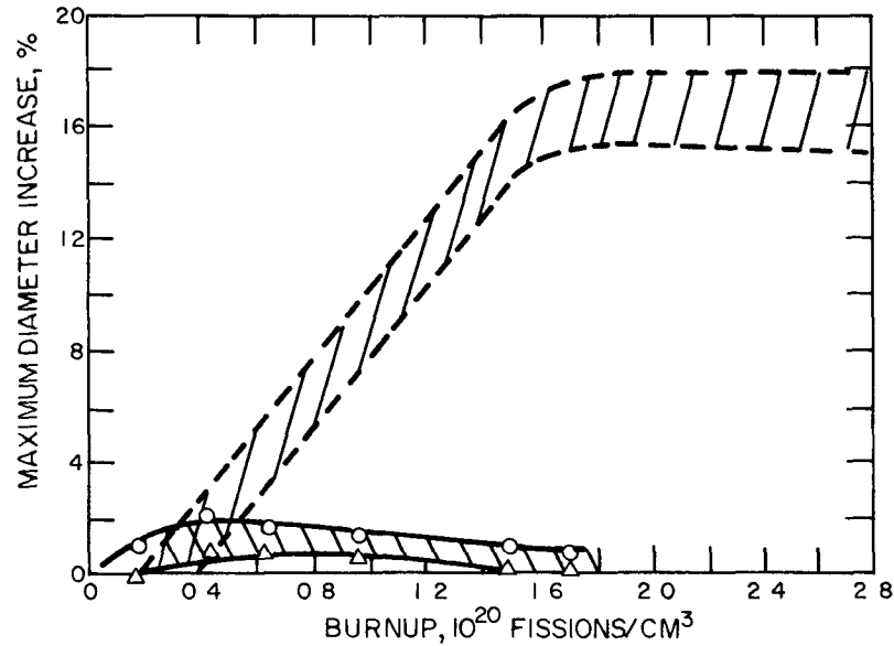
Fig. I-8 Effect of burnup on diametral swelling of W-UO 2 cermet. 54 Surface temperatures for the cermet ranged from 1600 to 1800°C. ZZZ , W-50 vol. % UO 2 , 20-mil cladding; o , W-42 vol. % UO 2 , 28% porosity 40-mil cladding, vented; Δ , W-42 vol. % UO 2 , 28% porosity, 40-mil cladding.
