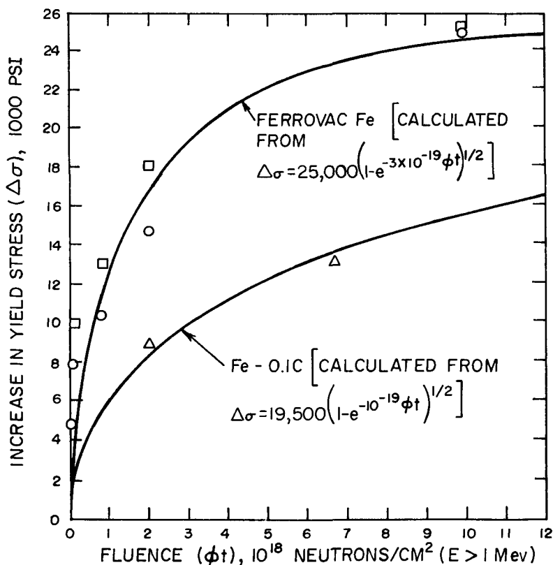
Fig. III-17 Comparison of predicted and measured irradiation-induced yield-strength changes in iron irradiated at 50 to 100^\circ\text{C} . 80 \square, \Delta : \Delta\sigma measured at room temperature; \circ - \Delta\sigma measured at 145^\circ\text{K} .
