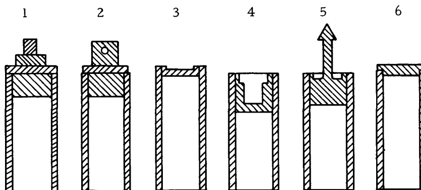
Types of End Caps
