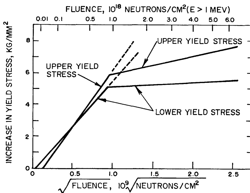
Fig. III-15 Effect of irradiation on yield stress of polycrystalline niobium. 69 (Irradiation temperature, < 50^\circ\text{C} ; test temperature, 25^\circ\text{C} ).
