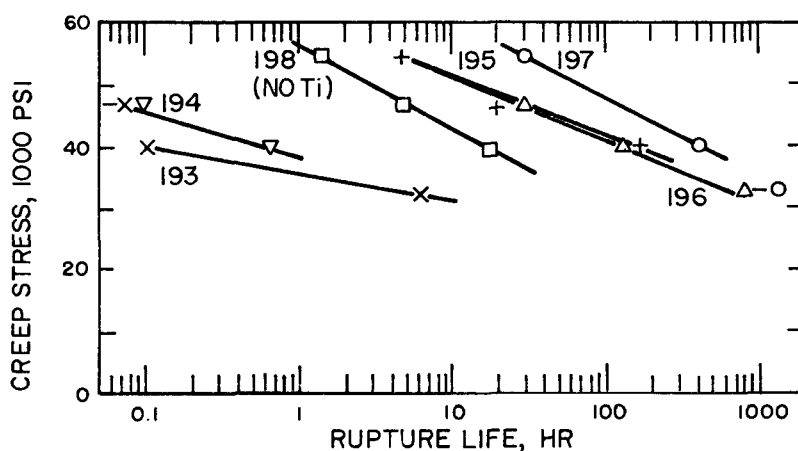
Fig. III-24 Effect of carbon on the rupture life of modified Hastelloy N at 650°C. 10b
