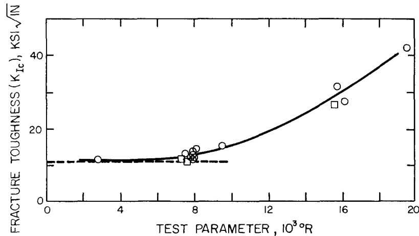
Fig. II-2 Effect of temperature and strain rate on fracture toughness of AMS 7902 beryllium. 13 ○, center-crack specimens; □, surface part-through specimens.
