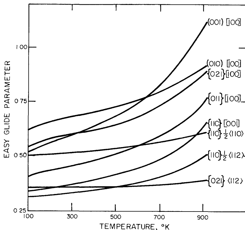
Fig. I-1. Temperature dependences of the easy-glide parameter for edge dislocations. 3
