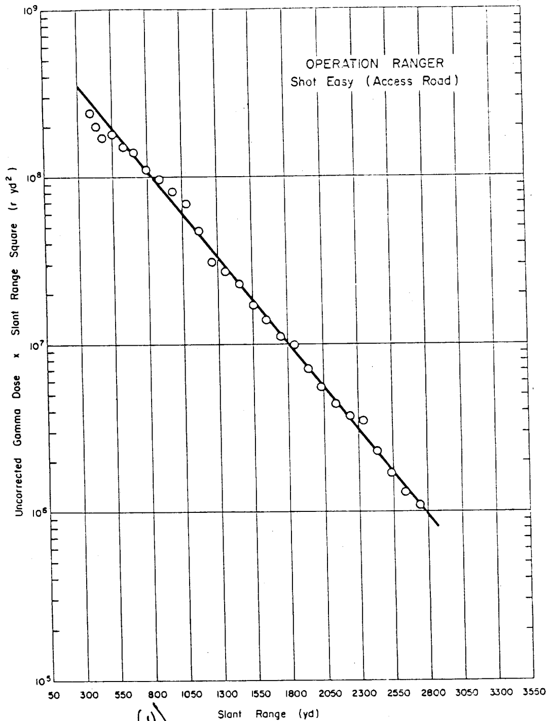
Figure 3.8 (U) (S-RD) Operation Ranger - Shot Easy (Access Road) - Uncorrected gamma-dose-times-slant-range- squared versus slant-range(U).
