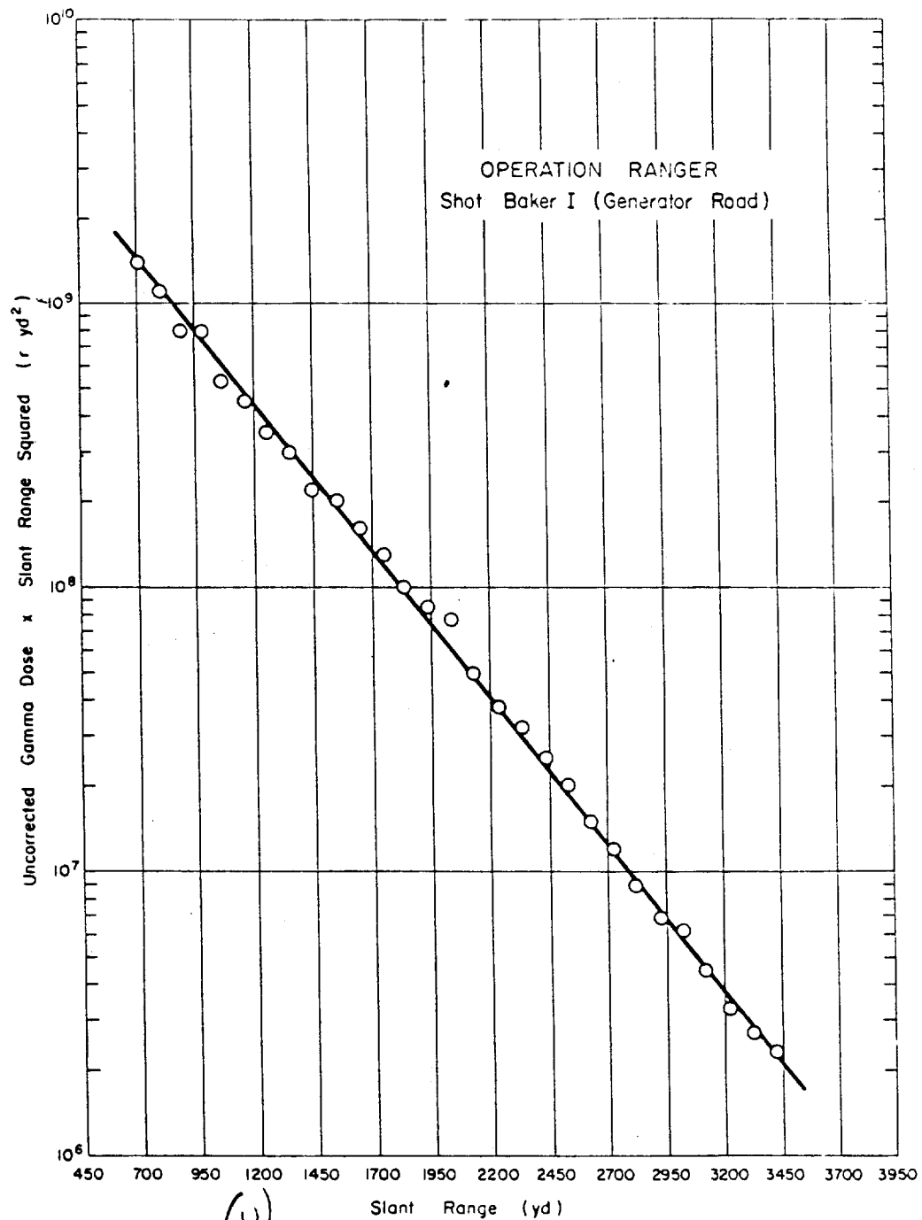
Figure 3.7 (S- RD ) Operation Ranger - Shot Baker I (Generator Road) - Uncorrected gamma-dose-times-slant-range-squared versus slant-range(U).
