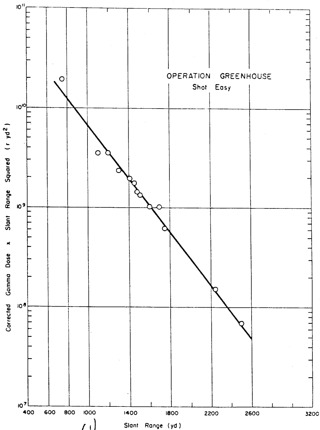
Figure 3.15 (S-RD) (U) Operation Greenhouse - Shot Easy - Corrected gamma-dose-times-slant-range- squared versus slant-range (U).
