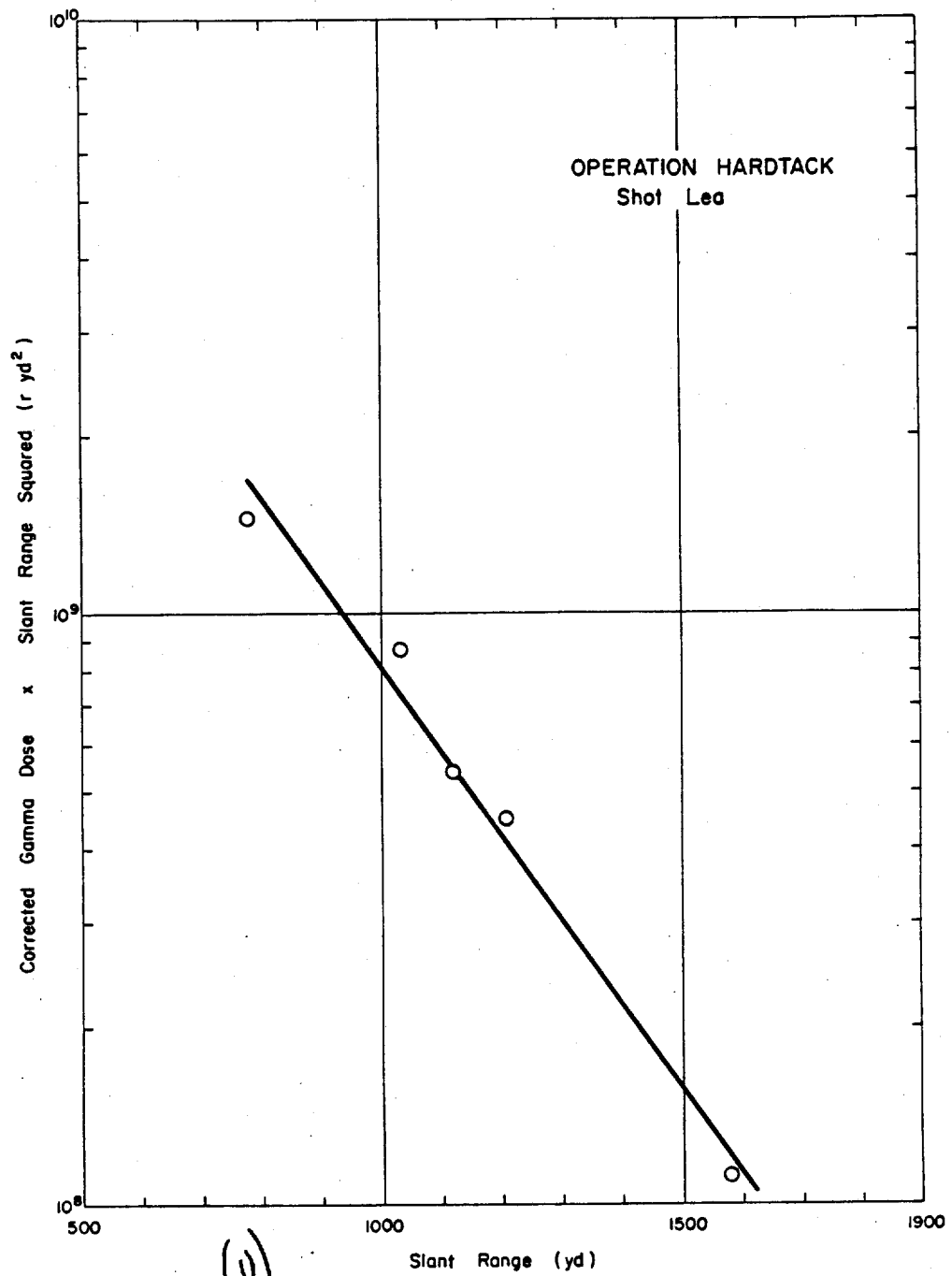
(U) Figure 3.84 (S-PD) Operation Hardtack - Shot Lea - Corrected gamma-dose-times-slant-range-squared versus slant-range (U).
