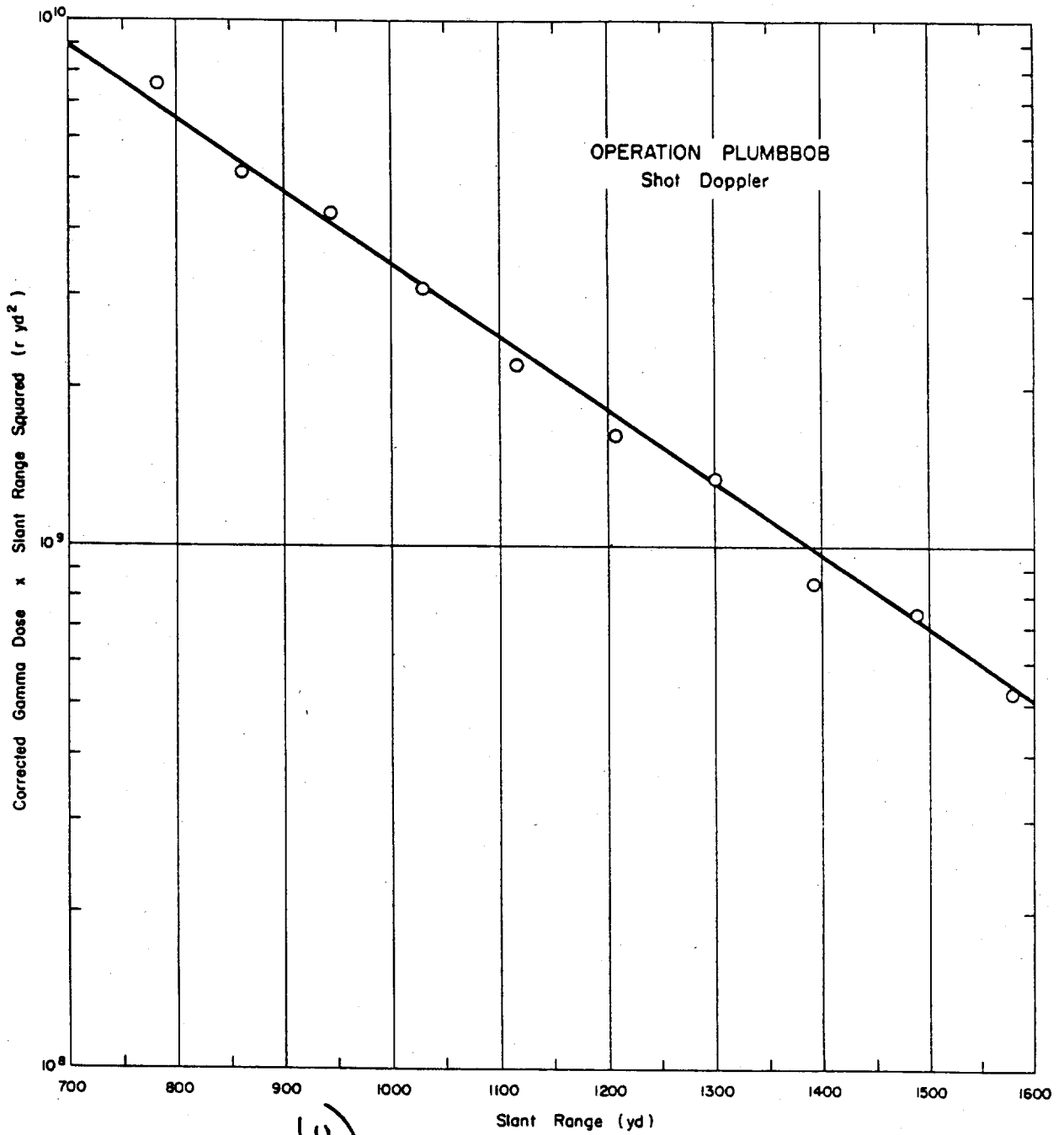
Figure 3.74 (U) (S-RD) Operation Plumbbob - Shot Doppler - Corrected gamma-dose-times-slant-range- squared versus slant-range (U).
