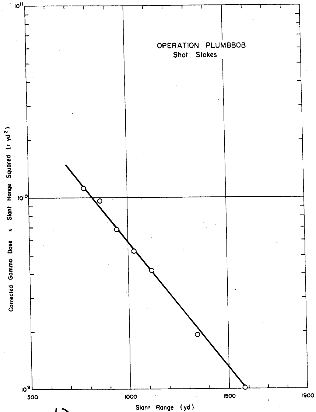
Figure 3.72 (S-2D) Operation Plumbbob - Shot Stokes - Corrected gamma-dose-times-slant-range-squared versus slant range (U).
