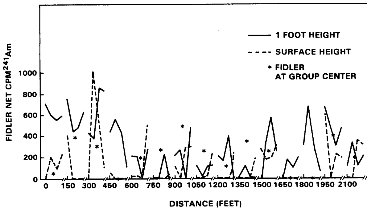
Figure 17. FIDLER Net CPM ^{241}\text{Am} Readings on Line 2 in Area 13, Project 57.
