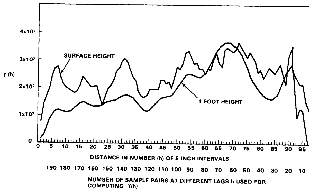
Figure 14. Variogram of Adjacent FIDLER Net CPM Am Readings Along Line 1 in Area 13, Project 57.
