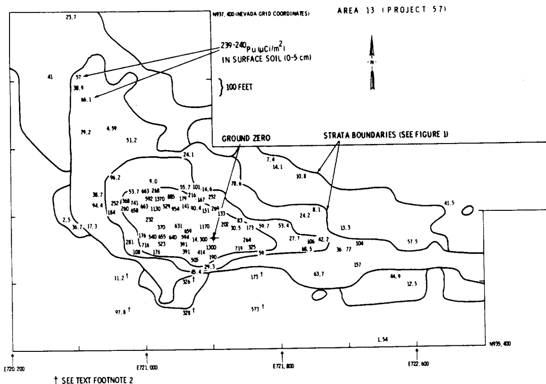
Figure 4. Observed ^{239-240}\text{Pu} Concentrations ( \mu\text{Ci}/\text{m}^2 ) in Surface Soil (0-5 cm) Within the 100-x 100-Foot Grid Area at the Project 57 (Area 13) Site.
