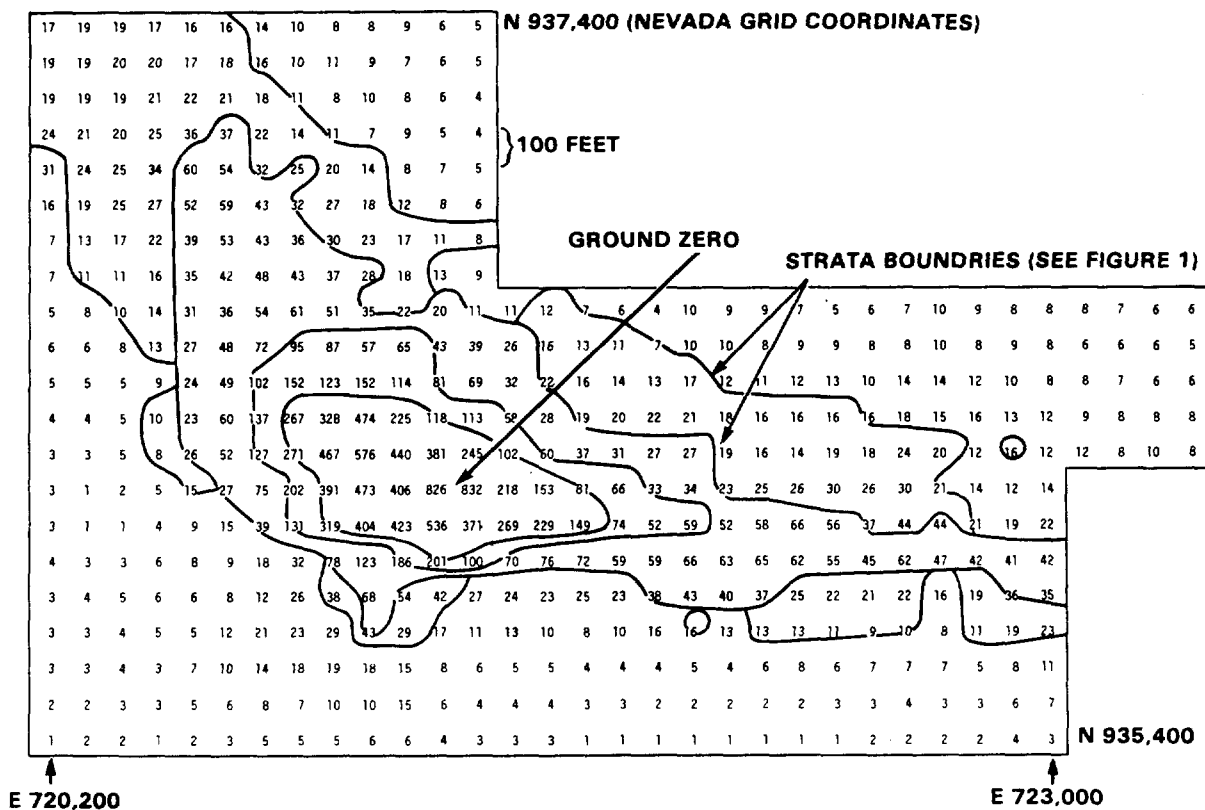
Figure 12. Estimate Arithmetic Mean Block Pu Concentrations ( \mu\text{Ci}/\text{m}^2 ) Using Equation 14 Ignoring 10^{\text{m}}/10^{\text{m(v)}} , or Equivalently, The Product of Formulae 15 and 16.
