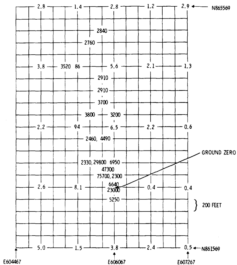
Figure 4. ^{239-240}\text{Pu} Concentrations (pCi/g) in Surface (0-5 cm) Soil at Nuclear Site-201 (Concentrations are for < 2 mm soil; No ball-milling was done).
