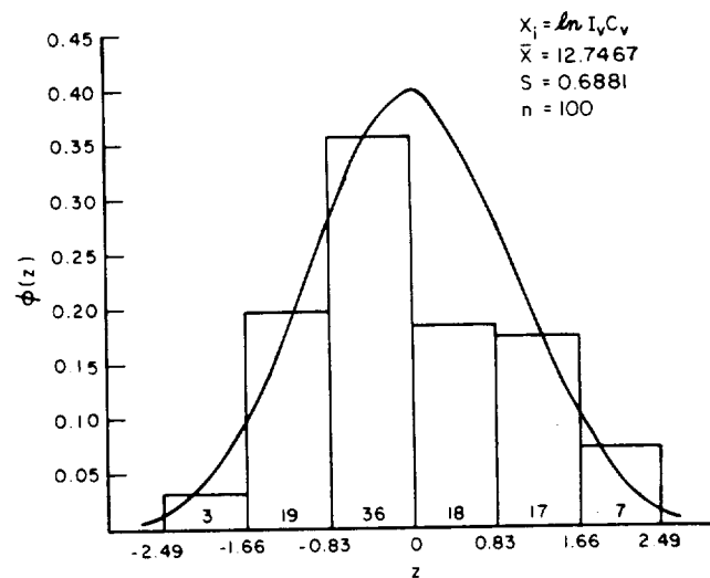
FIGURE 6. LOGNORMAL DISTRIBUTION OF PLUTONIUM UPTAKE FROM VEGETATION BY GRAZING CATTLE (Synthetic Composite Random Sample)
