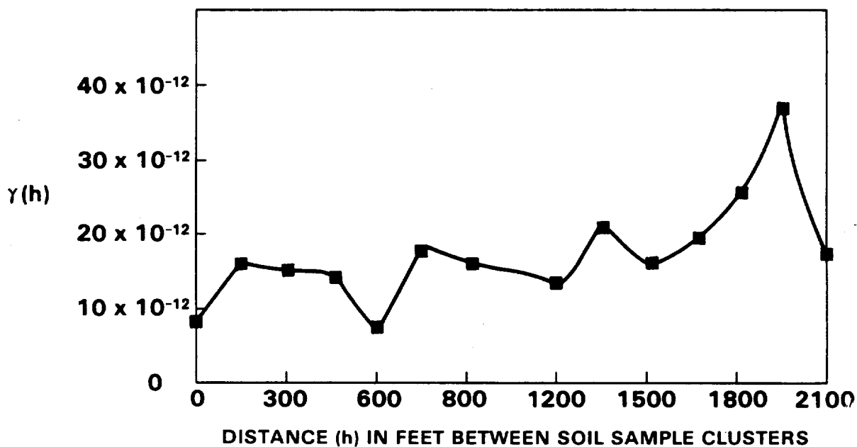
Figure 16. Estimated Raw Variogram of Line 2 ^{241}\text{Am} Concentrations.
