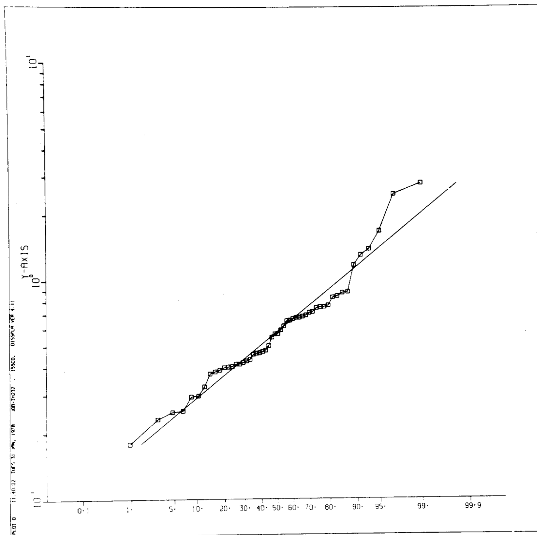
Figure 5. Log-Normal Plot of Th-232 Air Concentrations
