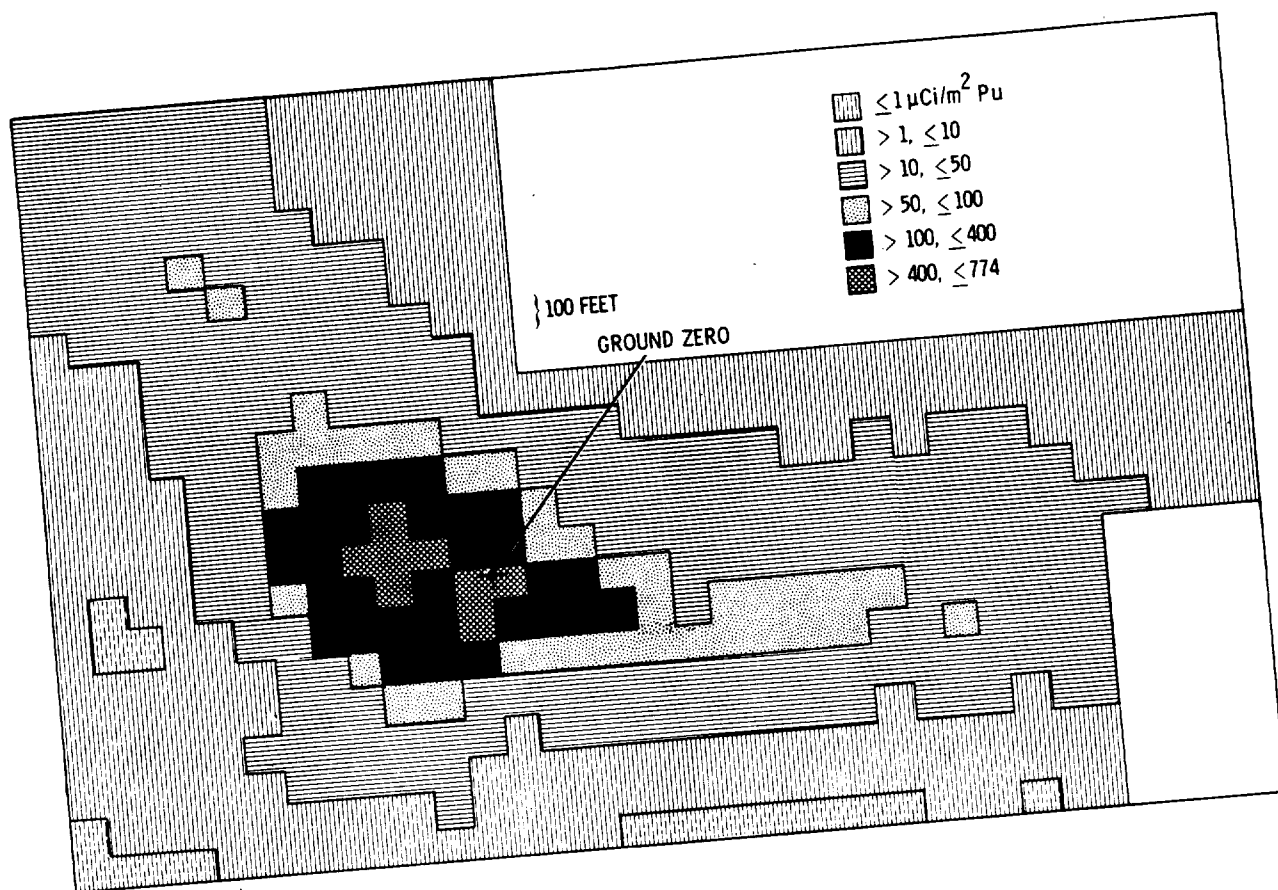
Figure 13. Estimated Geometric Mean Block Pu Concentrations 10^{P^*(v)} Using Equation 17.
