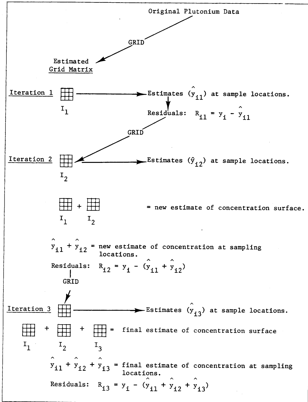
Figure 2. Iterative Procedure
