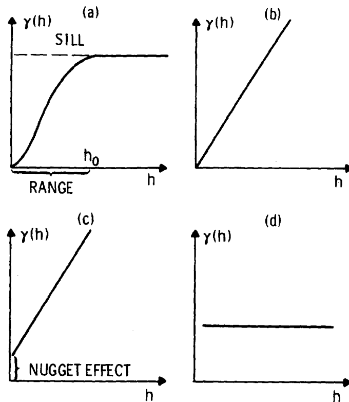
Figure 7. Theoretical Variograms.
