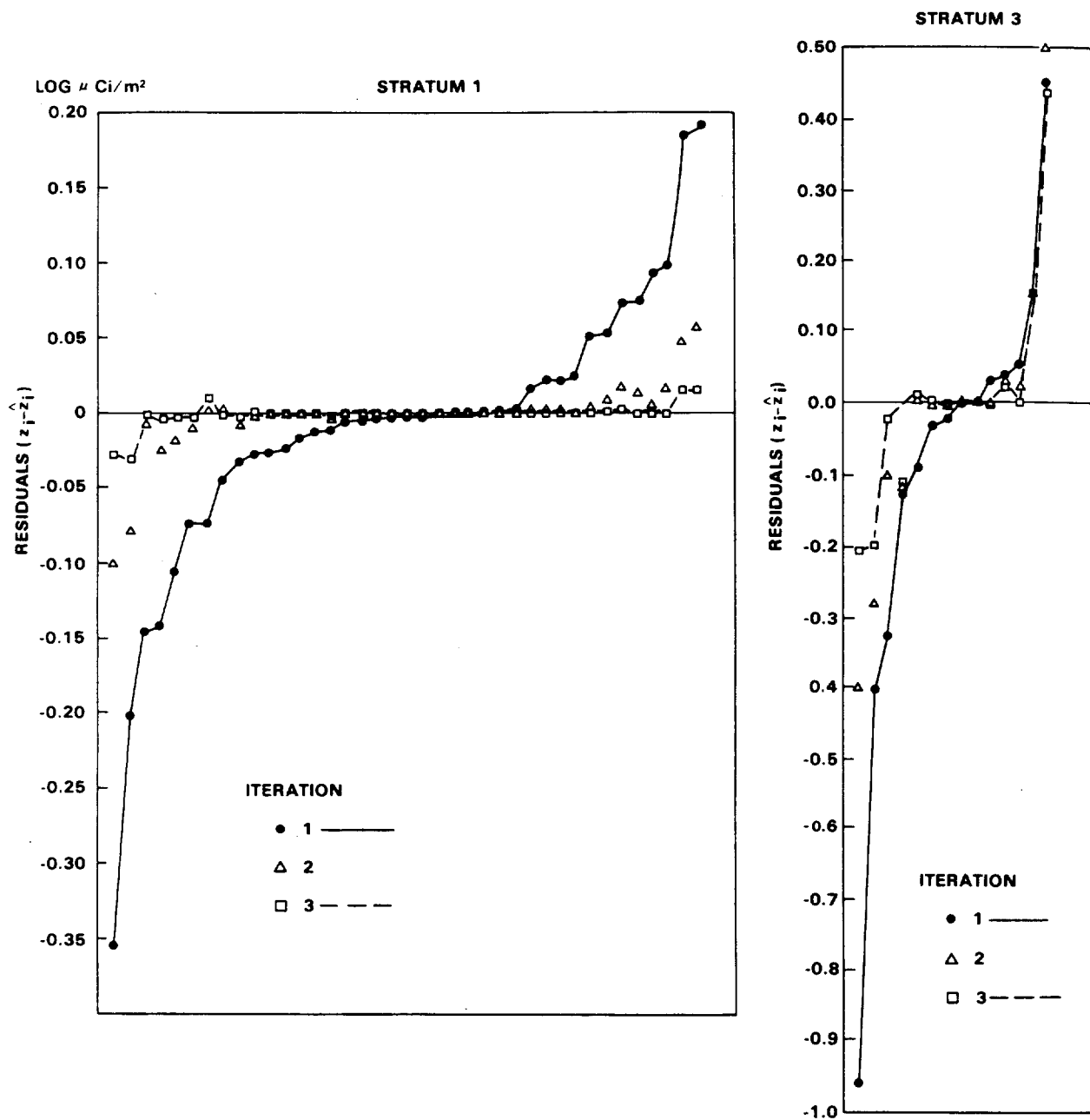
Figure 16. Residuals From Fitted Log 239-240 Pu Concentration Surface For Strata 1 and 3.
