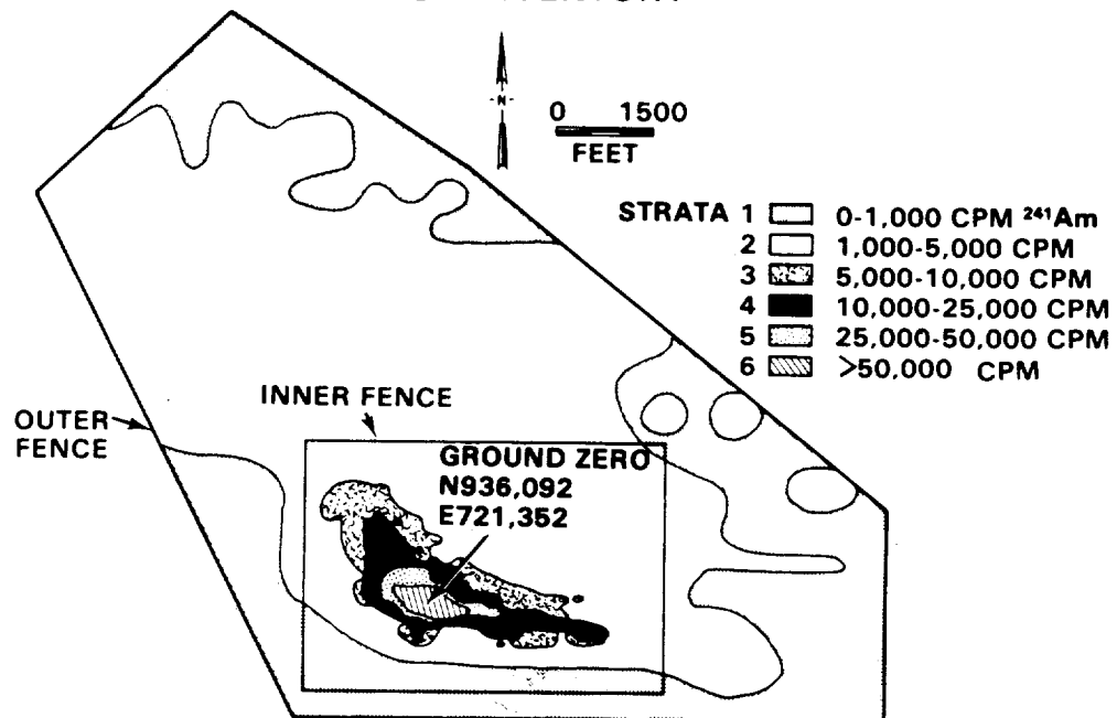
Figure 1. Area 13, Project 57-- ^{241}\text{Am} Activity Strata Obtained From FIDLER Grid Surveys (see Figure 2).
