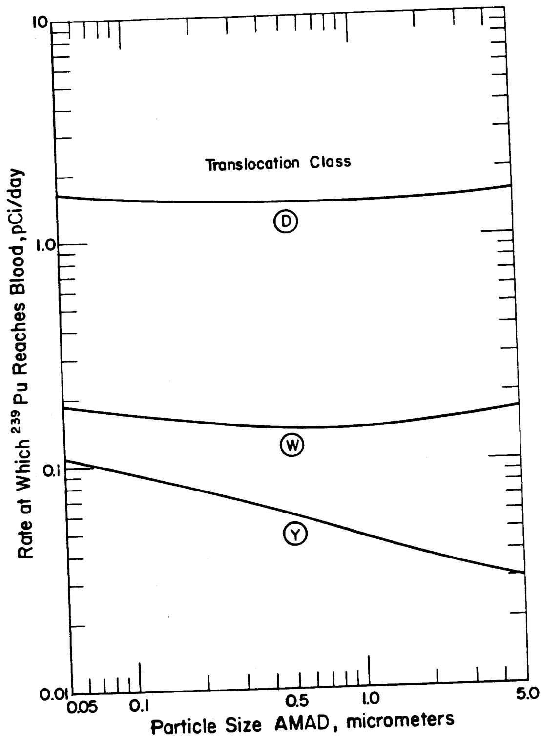
FIGURE 8. RATE AT WHICH ^{239}\text{Pu} REACHES BLOOD FROM INHALING 1 pCi/DAY AND INGESTING 1000 pCi/DAY ( H_m/A_m = 1000 )
