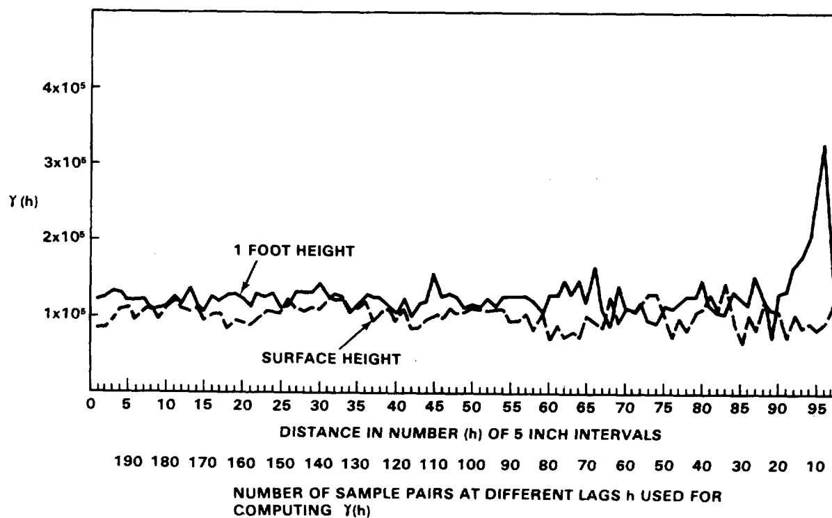
Figure 20. Variogram of Adjacent FIDLER Net CPM ^{241}\text{Am} Readings Along Line 2 in Area 13, Project 57.
