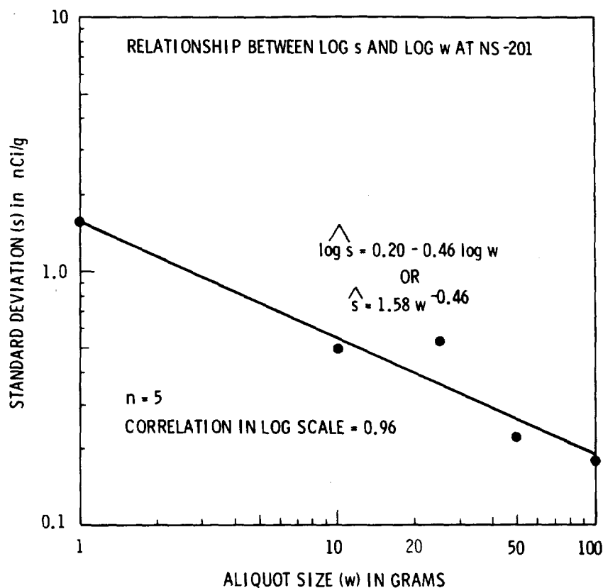
Figure 2. Estimated Relationship Between Log s and Log w for the Composite Soil Sample Collected Approximately 150 ft North of GZ at NS-201.
