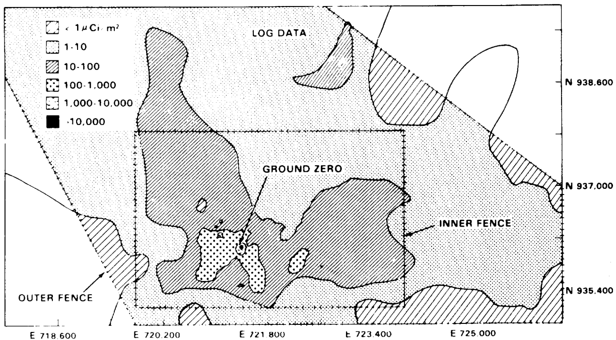
Figure 8. Estimated ^{239,240}\text{Pu} Concentration Contours in Surface Soil at the Area 13, Project 57 Site After 2 Iterations (Untransformed (Top) and Log Transformed (Bottom)).
