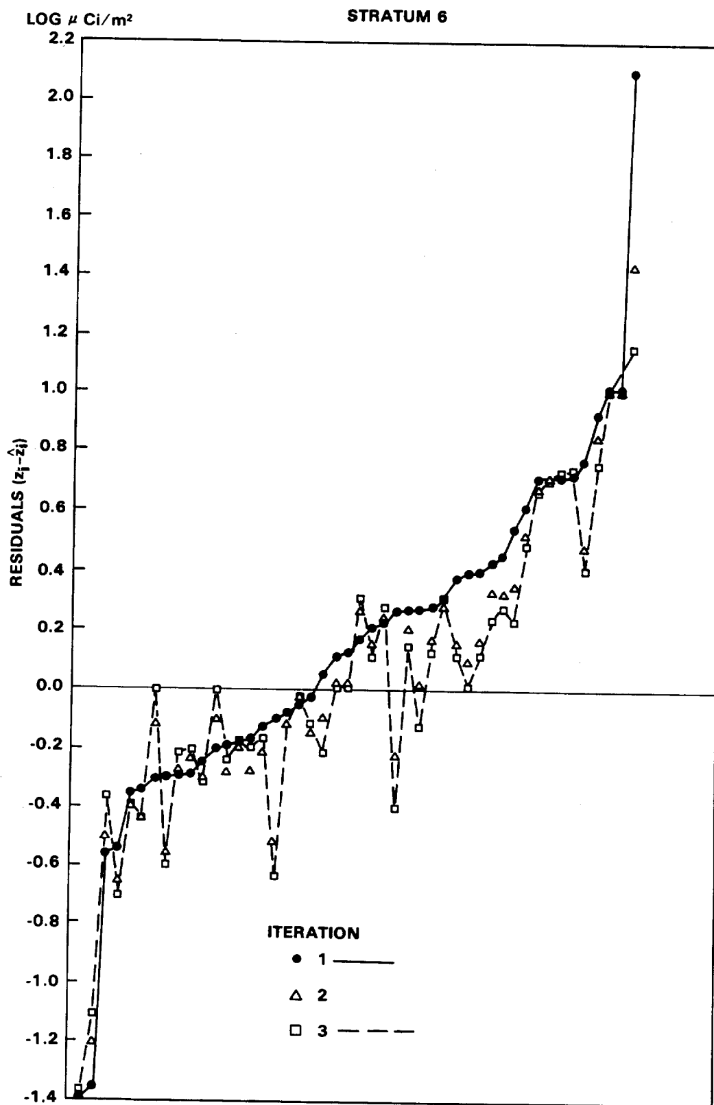
Figure 17. Residuals From Fitted Log ^{239-240}\text{Pu} Concentration Surface For Stratum 6.
