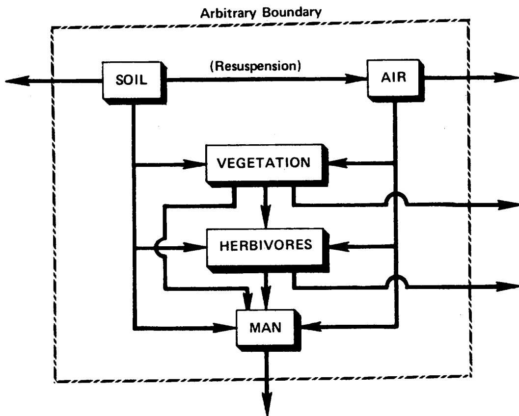
FIGURE 1. PRINCIPAL PATHWAYS OF PLUTONIUM TRANSPORT TO MAN
