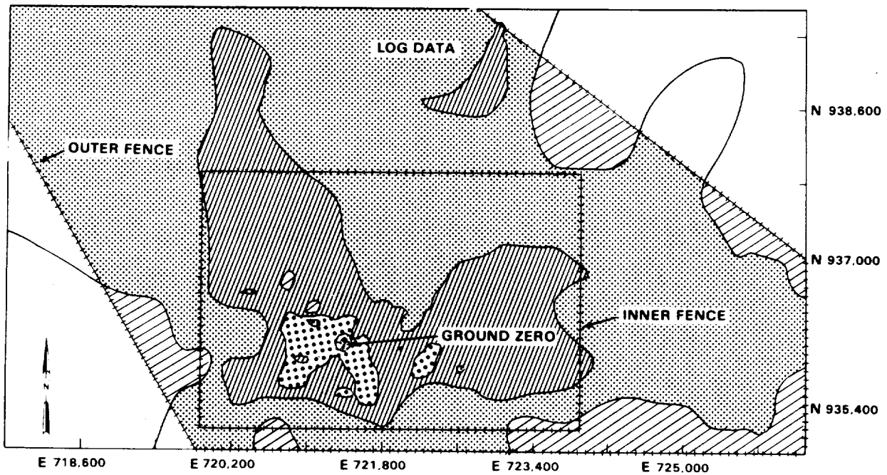
Figure 9. Estimated ^{239,240}\text{Pu} Concentration Contours in Surface Soil at the Area 13, Project 57 Site After 3 Iterations (Untransformed Data (Top) and Log Transformed (Bottom)).
