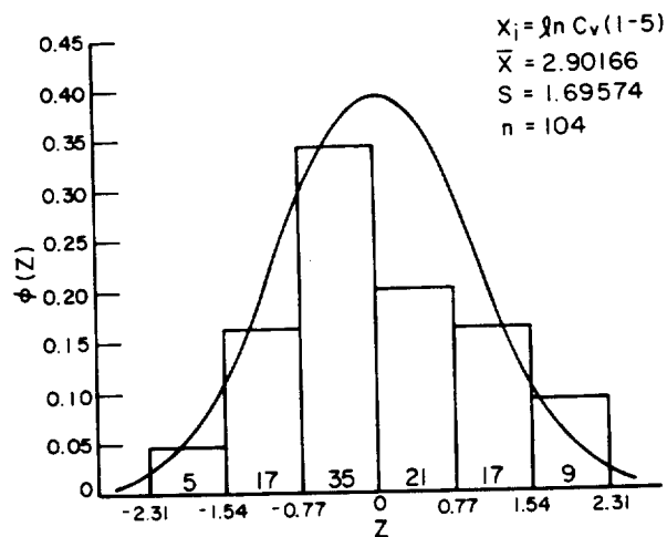
FIGURE 2. LOGNORMAL DISTRIBUTION OF PLUTONIUM (239-240) CONCENTRATIONS (pCi/g) IN VEGETATION SAMPLES FROM AREA 13 (NTS), STRATA 1-5
