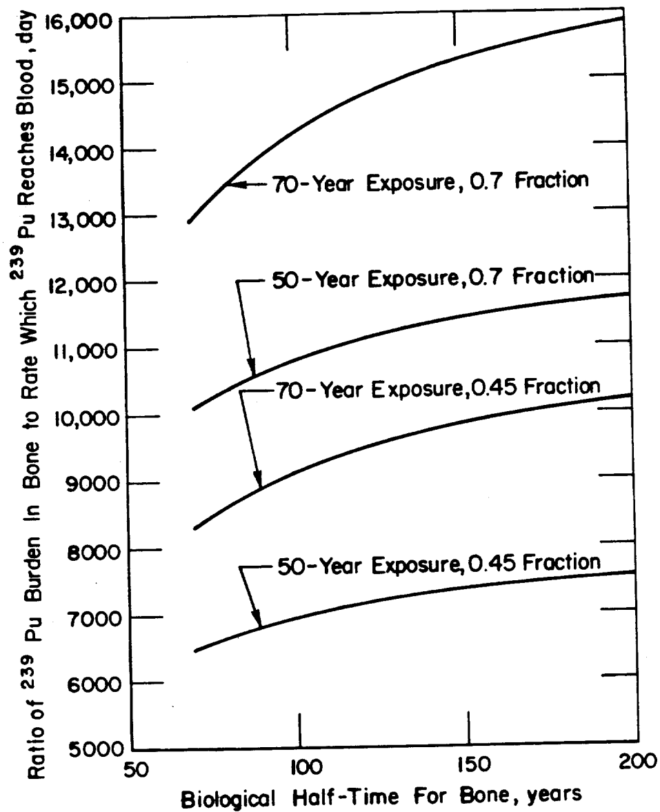
FIGURE 9. EFFECT OF BIOLOGICAL HALF TIME AND FRACTION FROM BLOOD TO BONE
