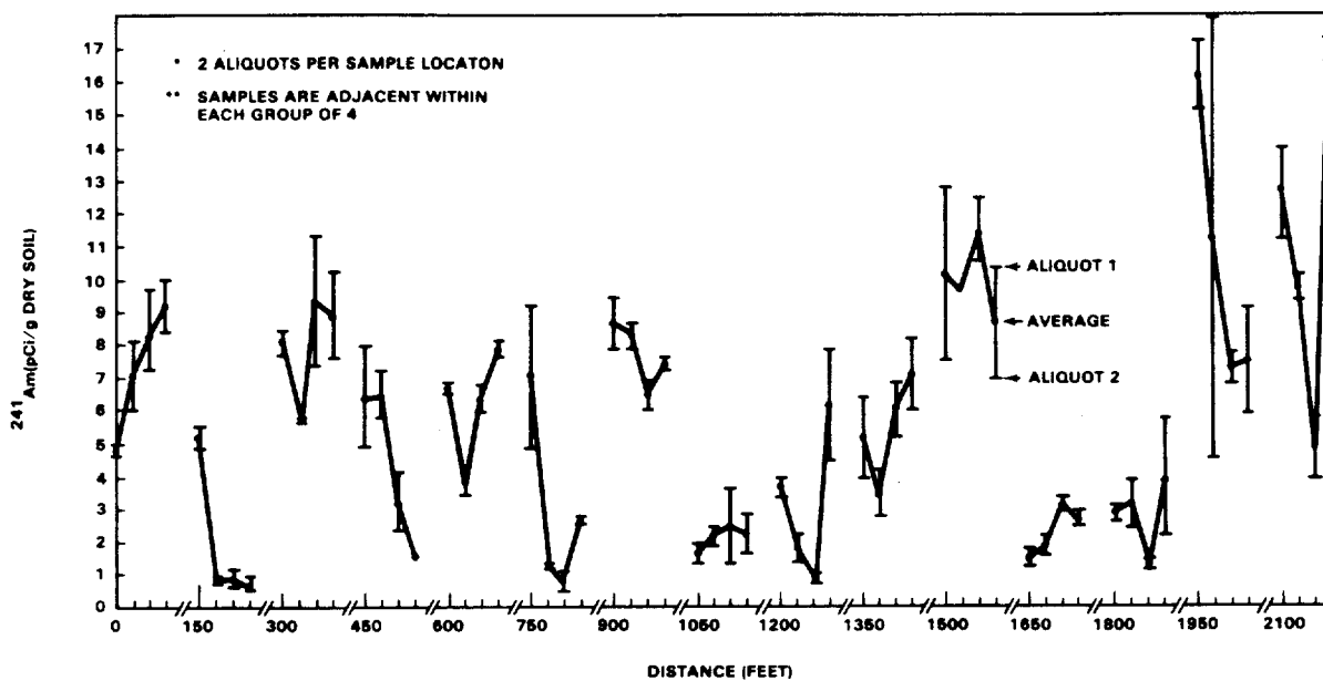
Figure 15. Average* Concentrations of ^{241}\text{Am} (pCi/g dry) in 70 g Aliquots of Soil Along Line 2** in Area 13, Project 57.
