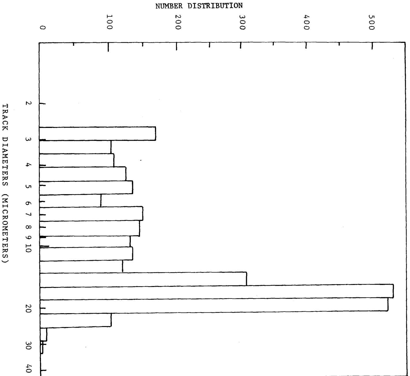
Figure 2. Distribution of track sizes in the exposed portion of film XXIX.
