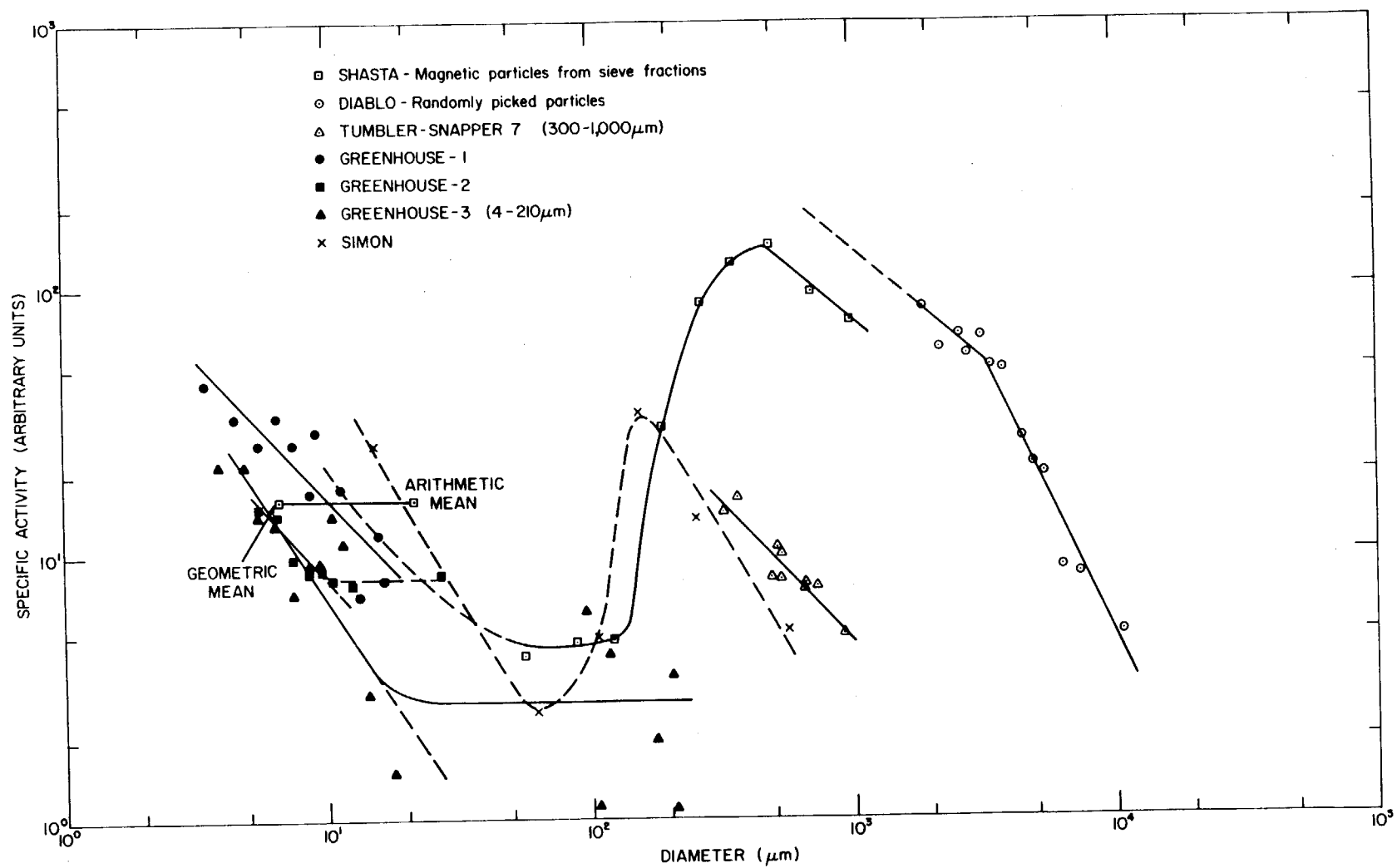
Figure 7. Specific Beta Activity of Particles from Several Tower Shots over a Large Size Interval.
