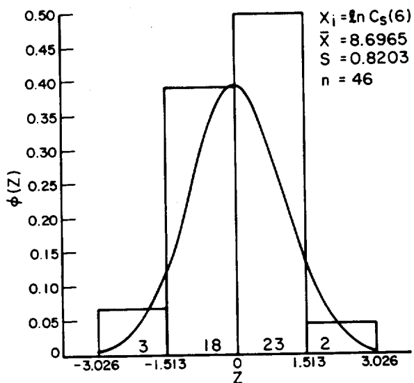
FIGURE 5. LOGNORMAL DISTRIBUTION OF PLUTONIUM (239-240) CONCENTRATIONS (pCi/g) IN SOIL SAMPLES FROM AREA 13 (NTS), STRATUM 6
