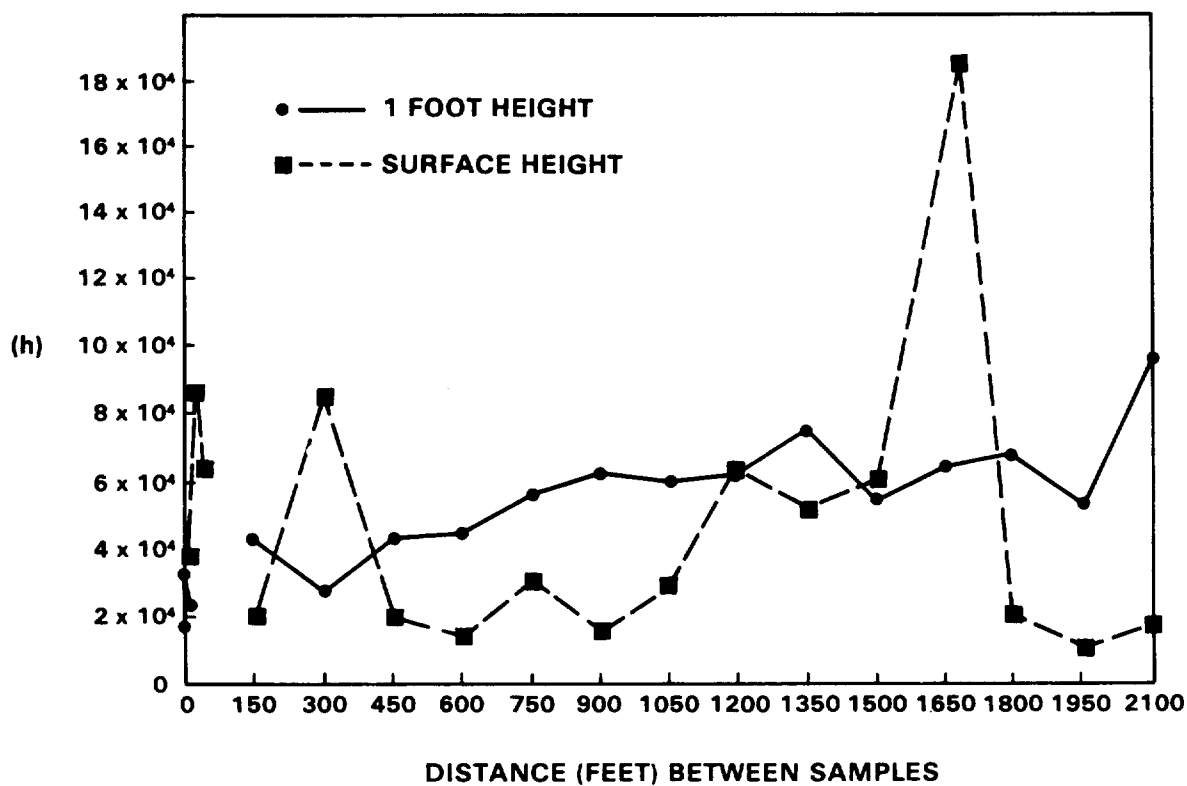
Figure 18. Estimated Raw Variograms of Line 2 FIDLER Data.
