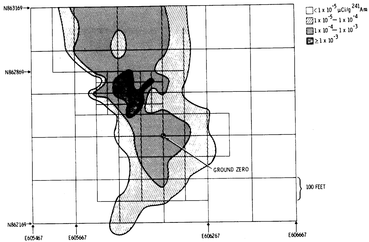
Figure 1. Hand Drawn Concentration Contours of ^{241}\text{Am} Near Ground Zero at Nuclear Site-201.
