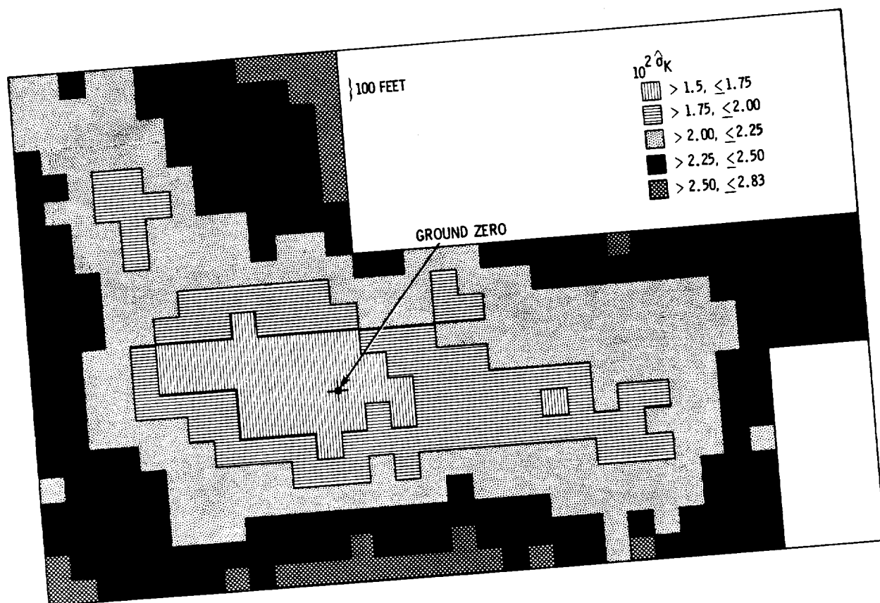
Figure 15. Contours of the Factor 10^{2\hat{\sigma}_K} for Obtaining an Approximate 95 Percent Confidence Interval for the Average Geometric Mean Concentration 10^P(v) .
