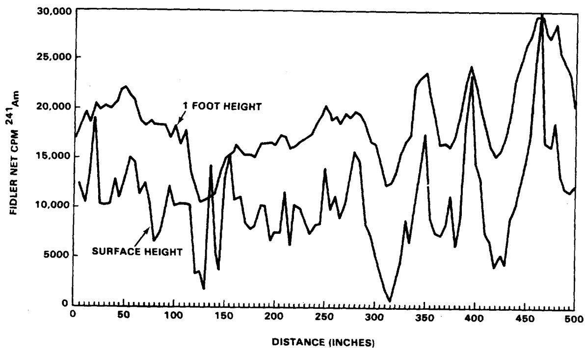
Figure 13. FIDLER Net CPM ^{241}\text{Am} (Average of Two Readings) at 5-in. Intervals Along Line 1 in Area 13, Project 57.
