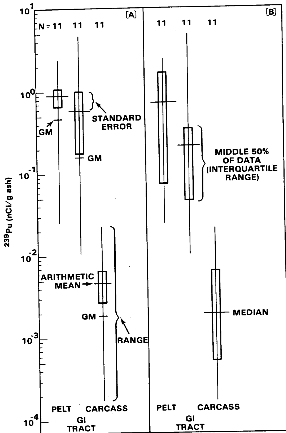
FIGURE 7. Three Sets of Rodent Data ( Dipodomys microps ) Summarized Two Different Ways: [A] Using Geometric Mean (GM), Arithmetic Mean, and Standard Error; [B] Using the Median and the Interquartile Range.
