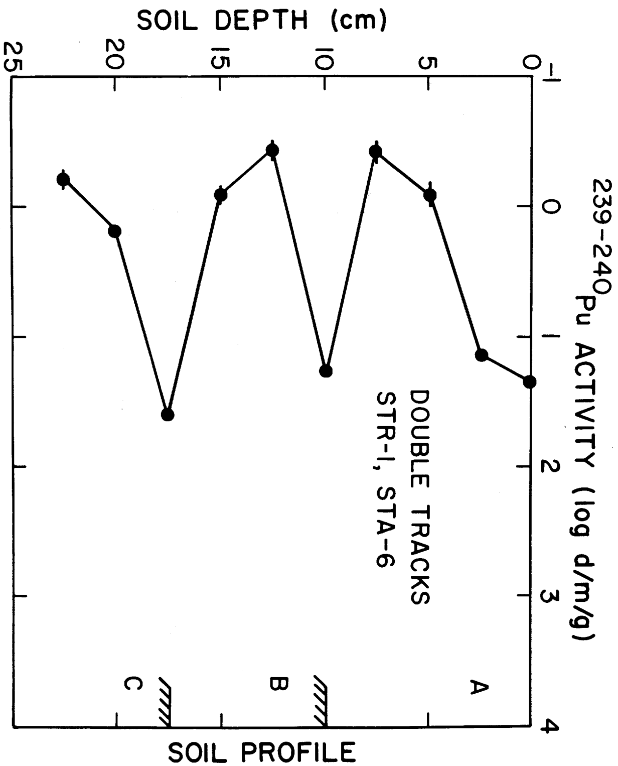
Fig. 2. Distribution of plutonium in Double Tracks soil profile with silicon/iron traces
