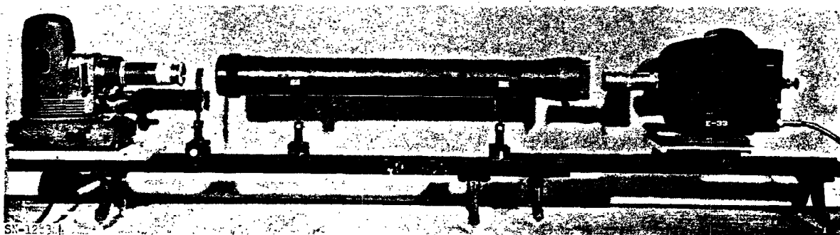
Fig. 6. Collimator setup for focal length measurements.
