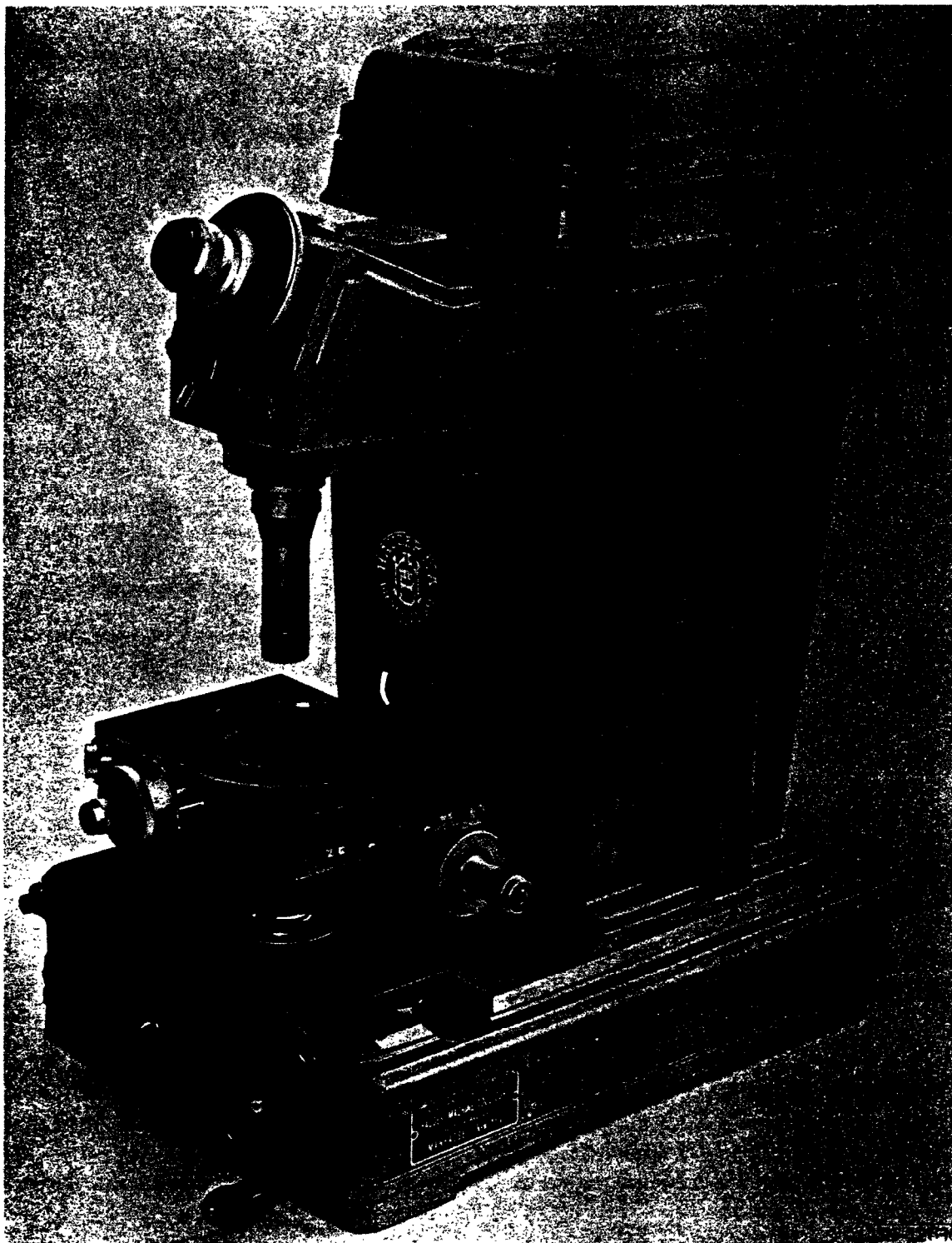
Fig. 12. Hauser profile measuring microscope, Model P219.
