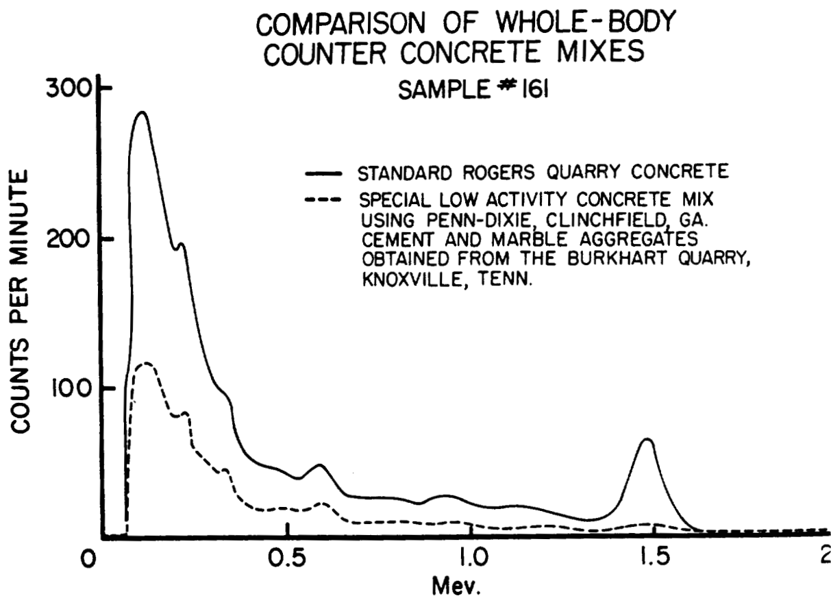
Fig. 3. Comparison of spectra of the locally available concrete mix and the special low-activity mix used in building the ORINS low-level whole-body counting facility.
