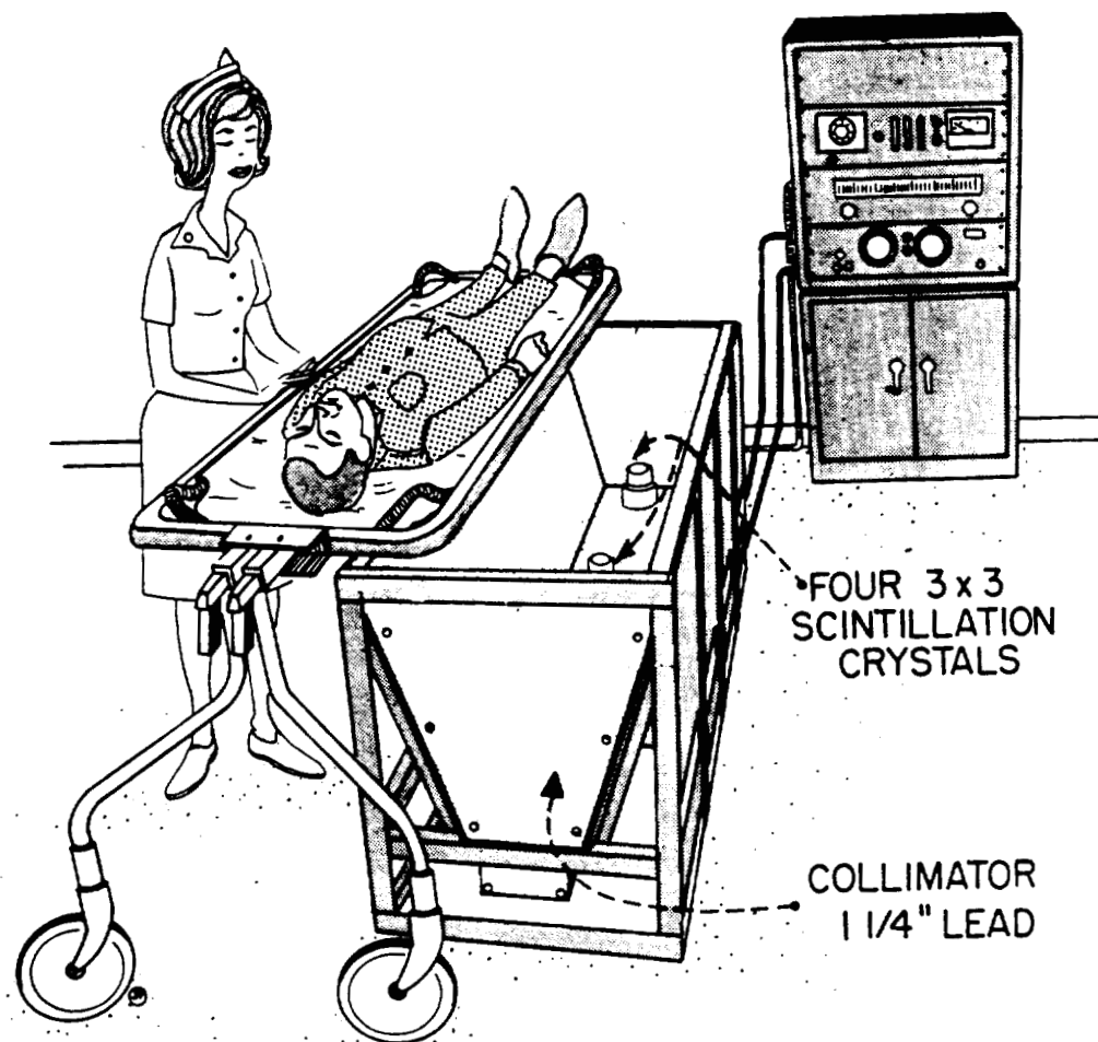
Fig. 2. The ORINS diagnostic-level whole-body counter.
