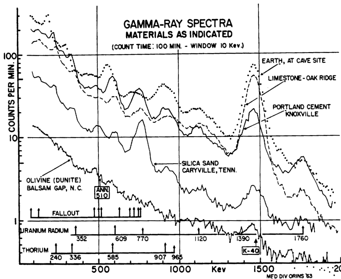
Fig. 3 Gamma-ray spectra for several materials, ranging from the "hot" earth at the construction site to the "cold" North Carolina olivine. The arrows near the bottom show the peak locations for a number of radionuclides of interest.
