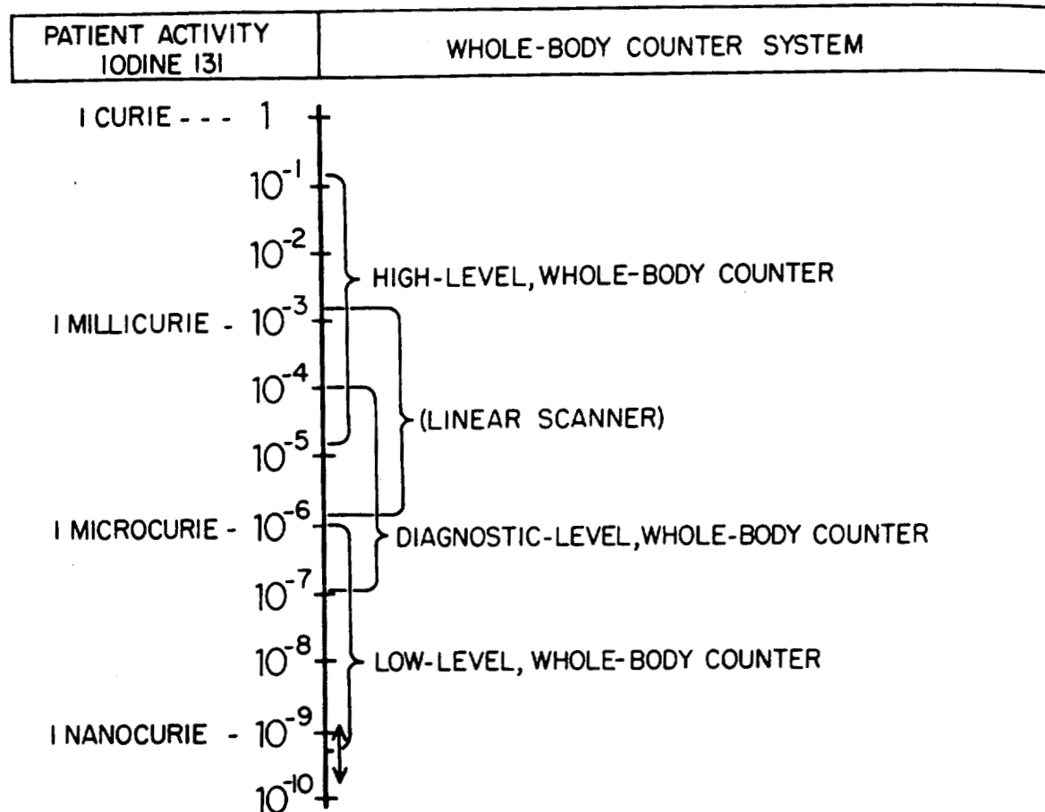
Fig. 1. Sensitivity ranges for the ORINS Whole-Body Counters.
