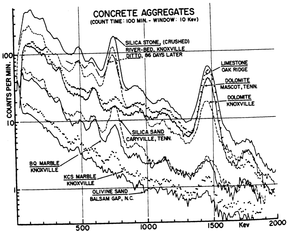
Fig. 6 Concrete aggregates. (See arrows at bottom of Fig. 3.)
