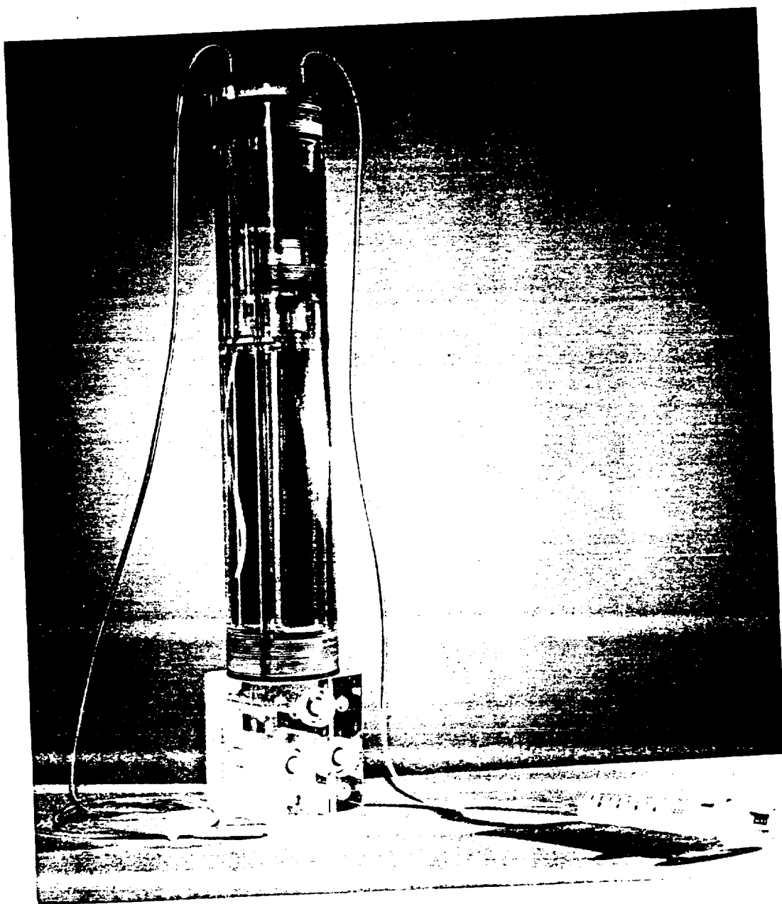
Fig. 1. ORINS arm counter.
