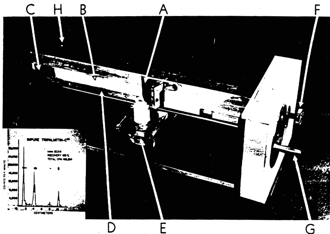
Fig. 1. Thin-layer chromatogram scraper.
