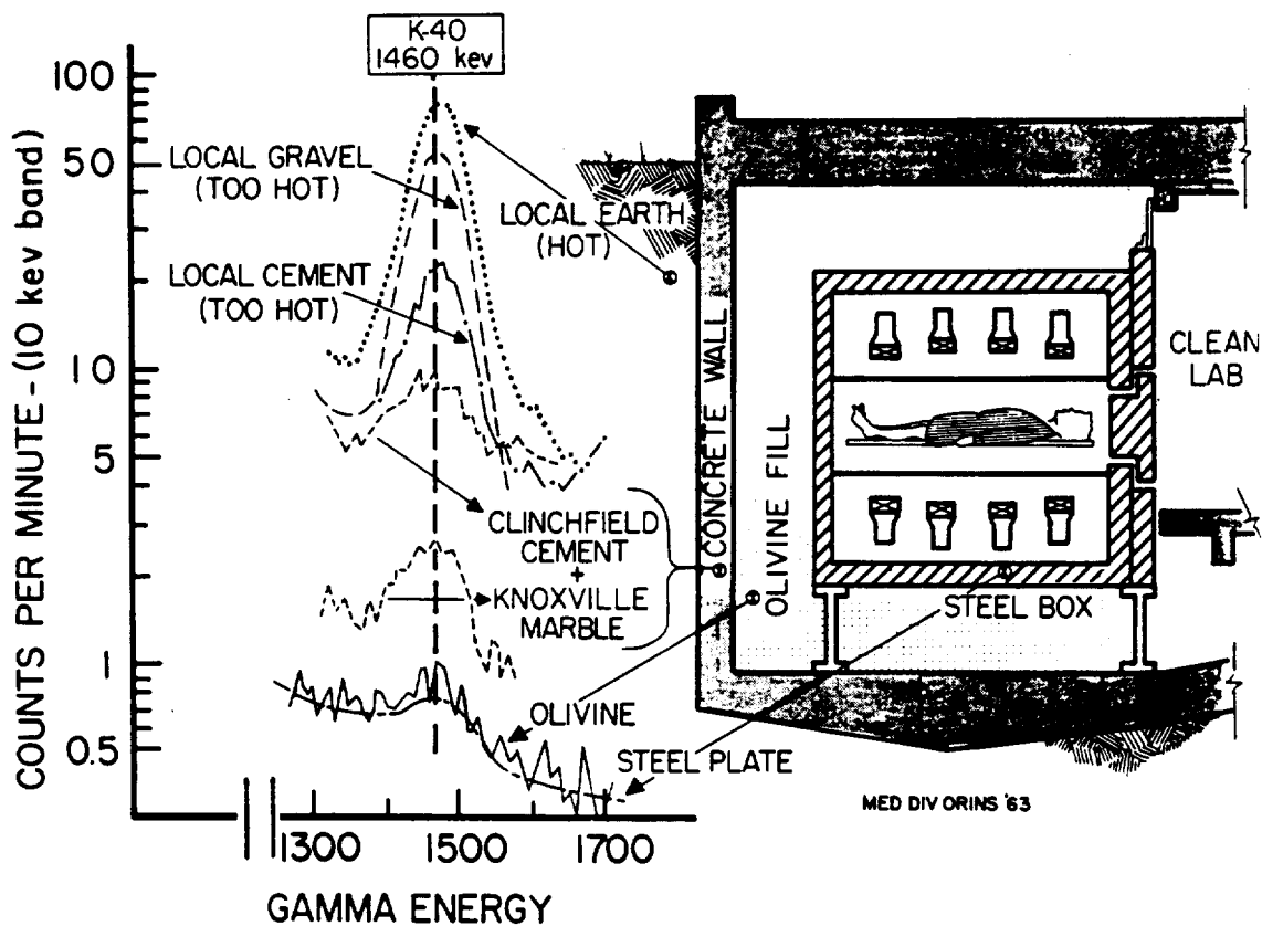
Fig. 9 Vertical section (schematic) through the patient-counting chamber, showing the wall structure. The K^{40} regions of the spectra are shown at the left, to indicate how the inherent radioactivity decreases progressively from the "hot" earth to the "cold" steel box.
