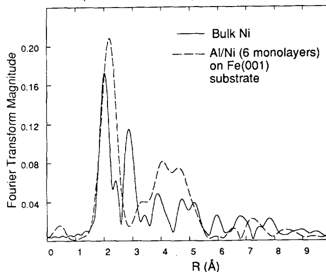
Comparison of 6 Monolayer and Bulk Nickel
