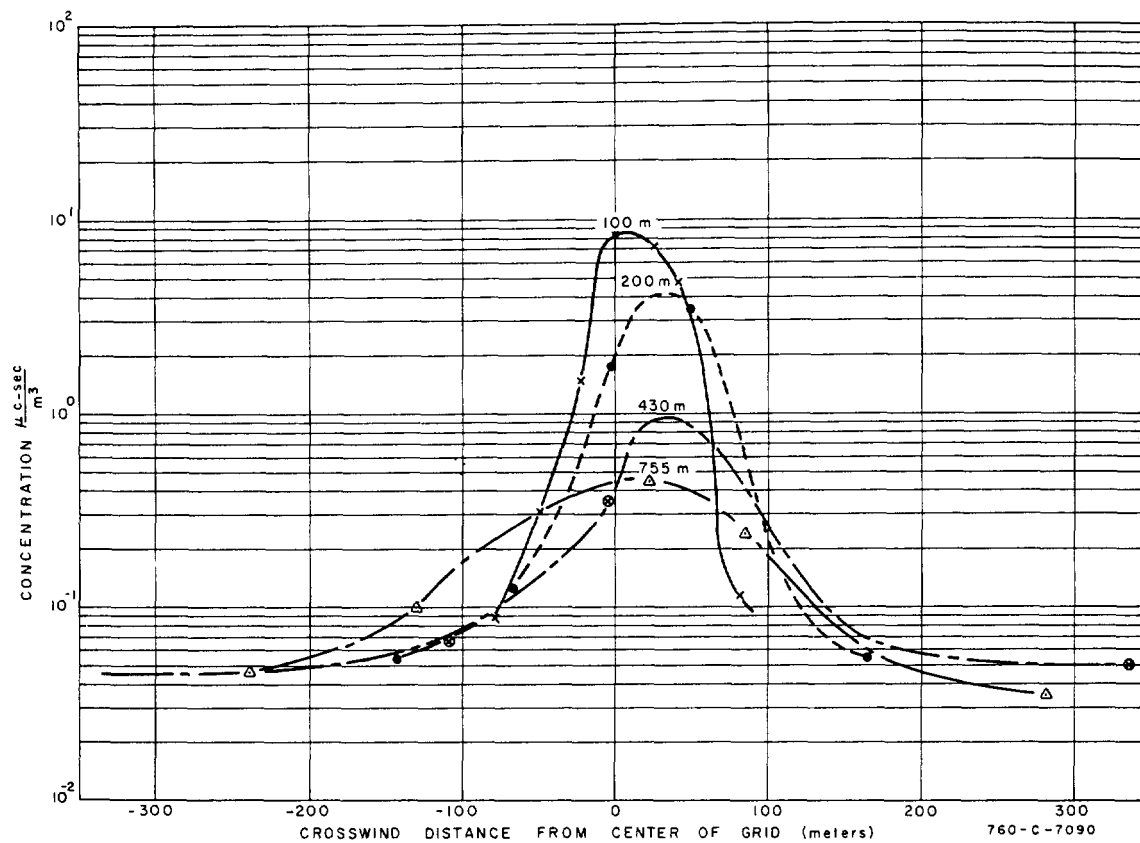
FIG. C-4 CROSSWIND CONCENTRATION CURVES FOR DOWNWIND DISTANCES FROM SECOND SPURT I DESTRUCTIVE TEST, NOVEMBER 10, 1963.
