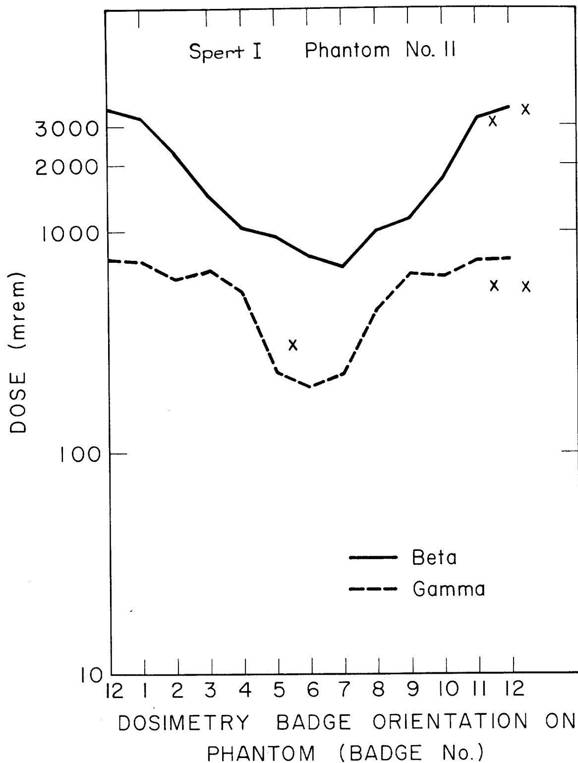
FIG. C-2 DOSE VS DOSIMETER BADGE ORIENTATION ON PHANTOM.
