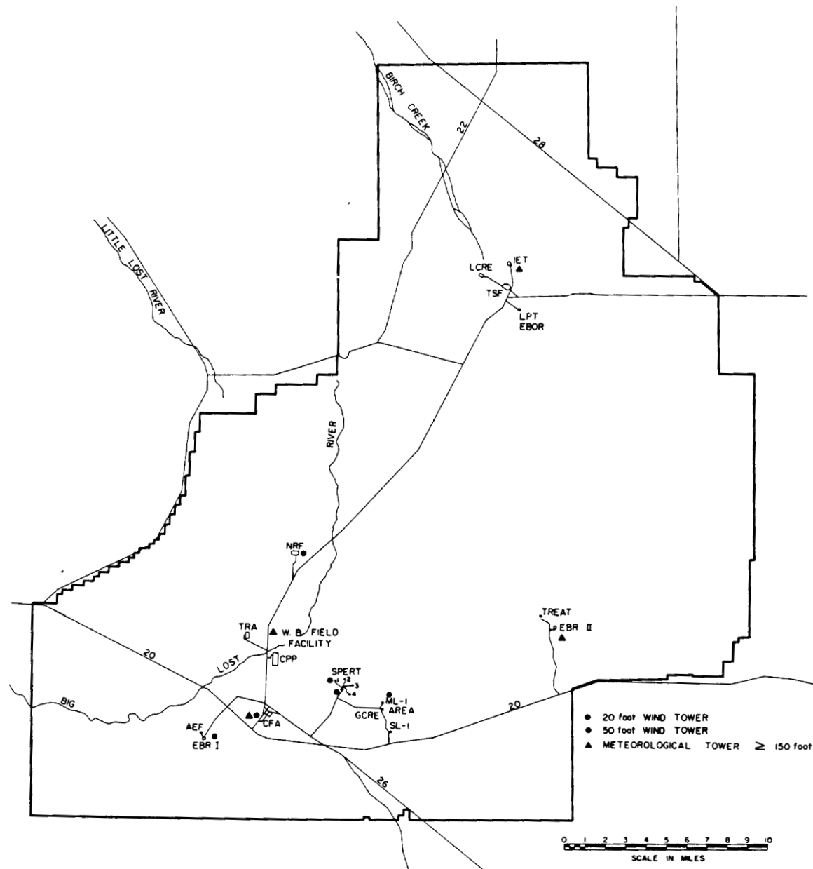
FIG. 11 LOCATIONS OF METEOROLOGICAL INSTRUMENTATION ON THE NATIONAL REACTOR TESTING STATION.
