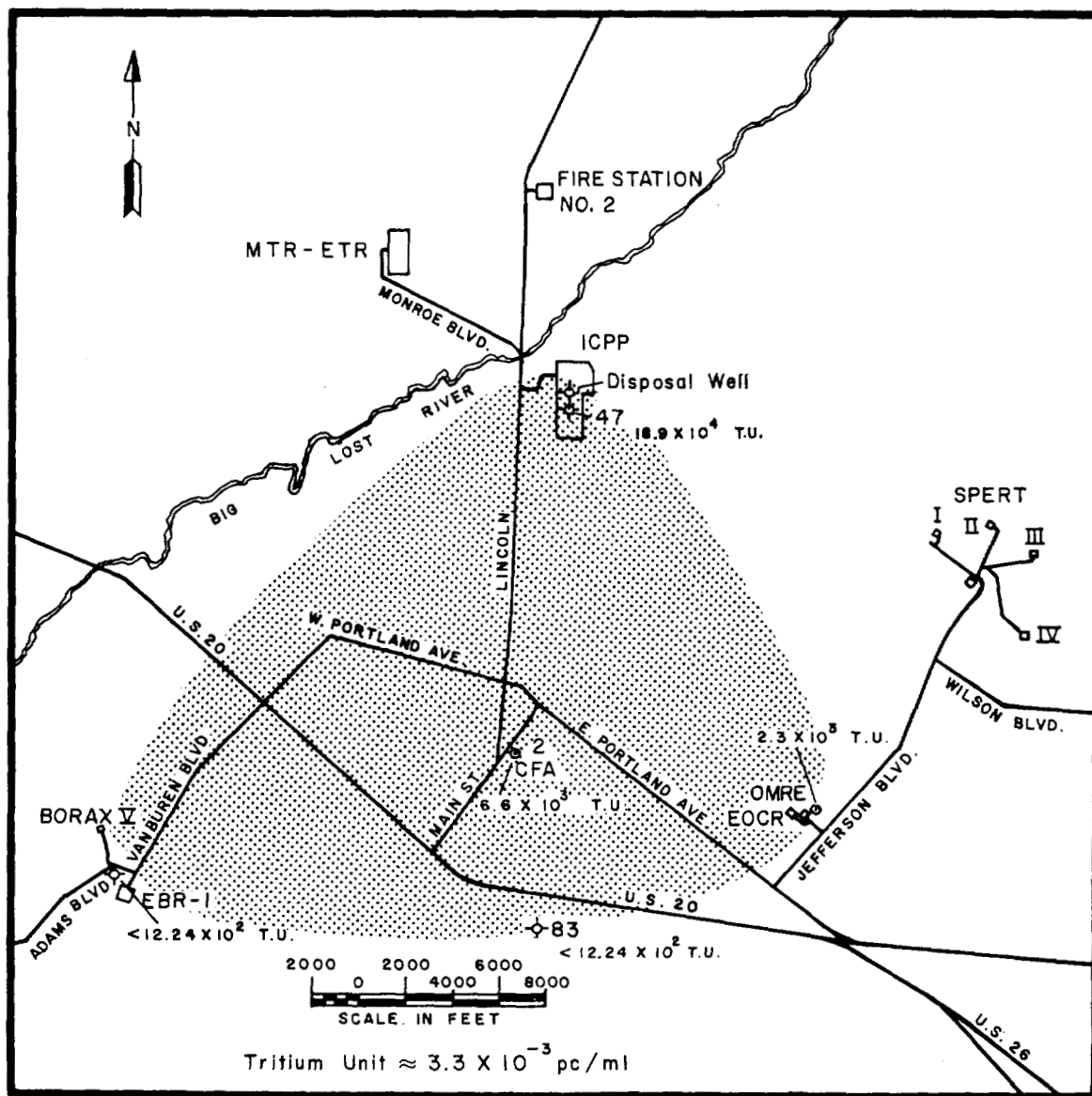
FIG. 8 TRITIUM IN GROUND WATER, ICPP - CFA
