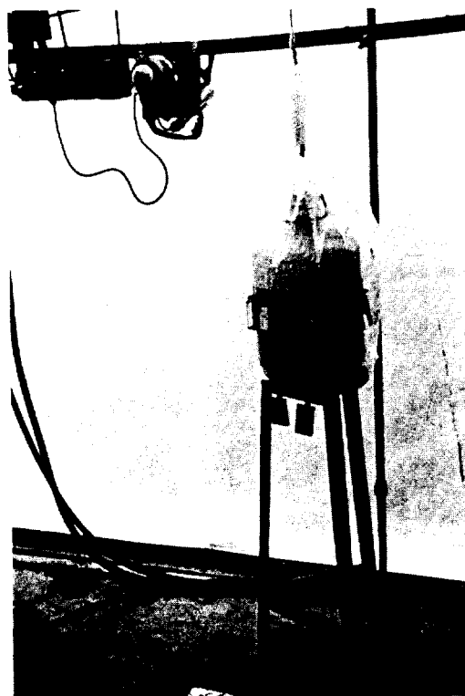
FIG. C-1 FILM DOSIMETERS ON STANDARD MAN PHANTOM.
