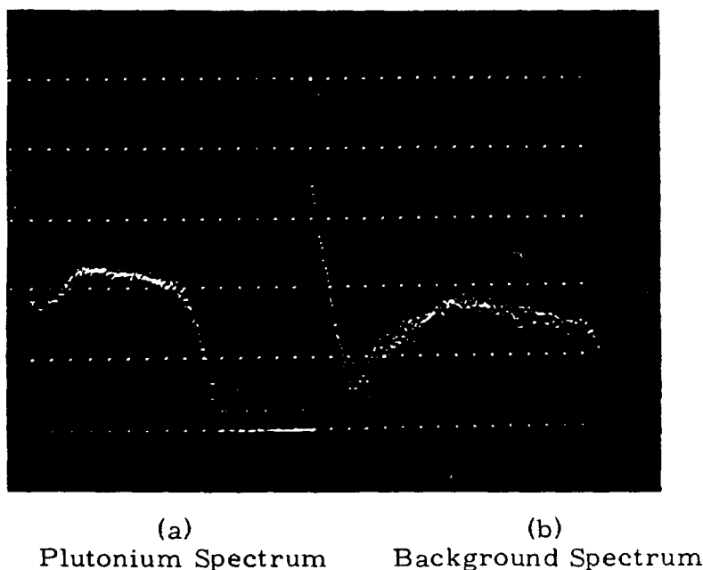
FIGURE 5.42 Typical Alpha Spectra
