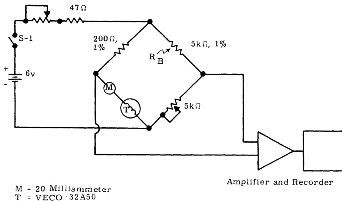
FIGURE 5.23 Thermistor Bridge
