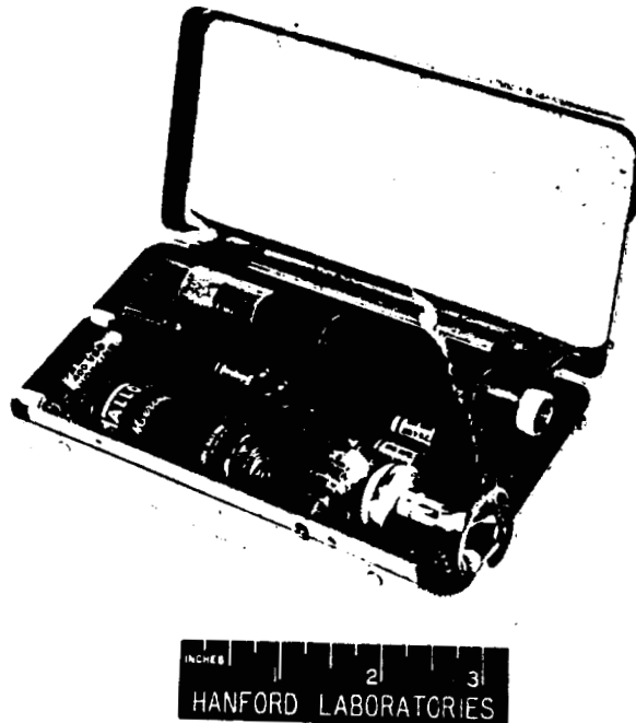
FIGURE 5. 40 Internal View of Completed Dosimeter
