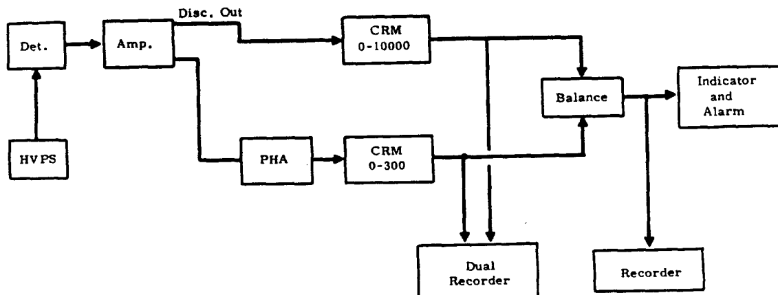
FIGURE 5.44 Block Diagram Alpha Energy Analysis Air Monitor
