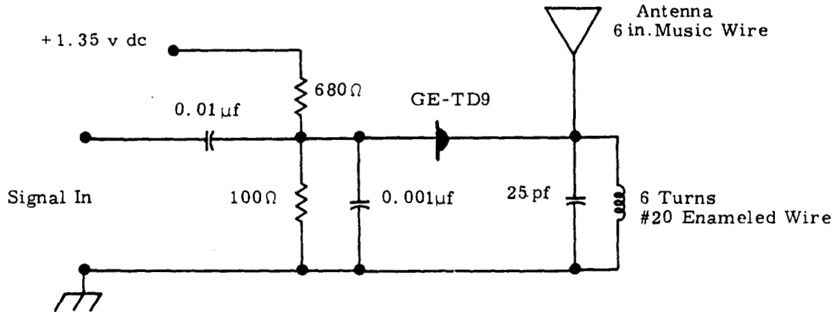
FIGURE 5.32 FM Transmitter
