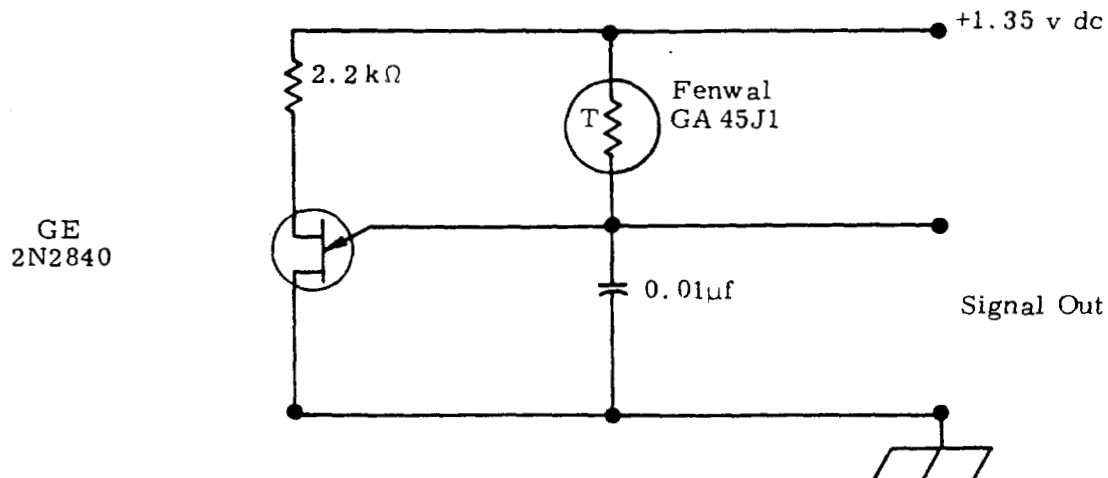
FIGURE 5.33 Temperature Transducer
