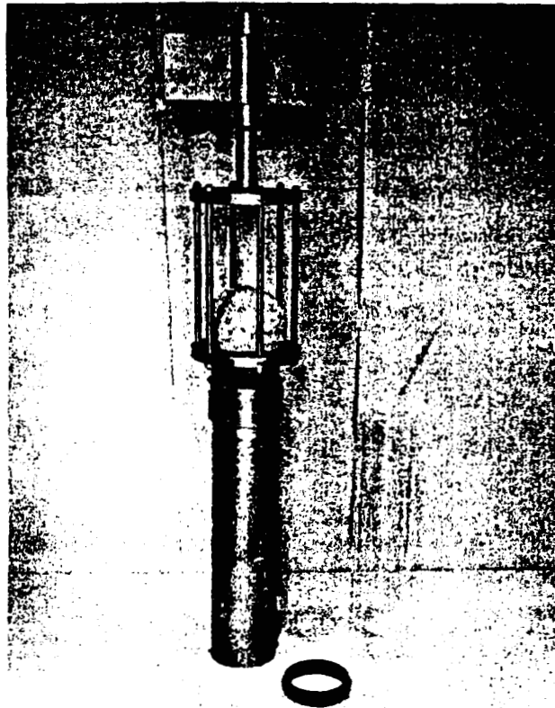
FIGURE 3.31 Core Sampler
