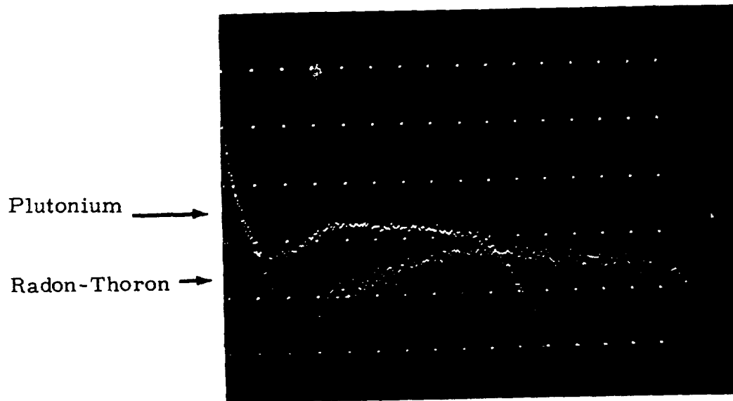
FIGURE 5.43 Spectra Superimposed
