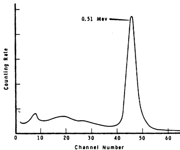
FIGURE 3.2 \text{Cu}^{64} Spectra
