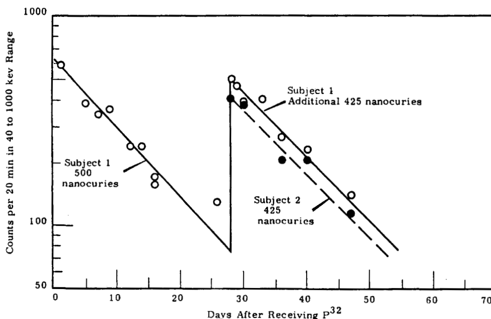
FIGURE 2.4 Retention of Low Level Burdens of P^{32}
