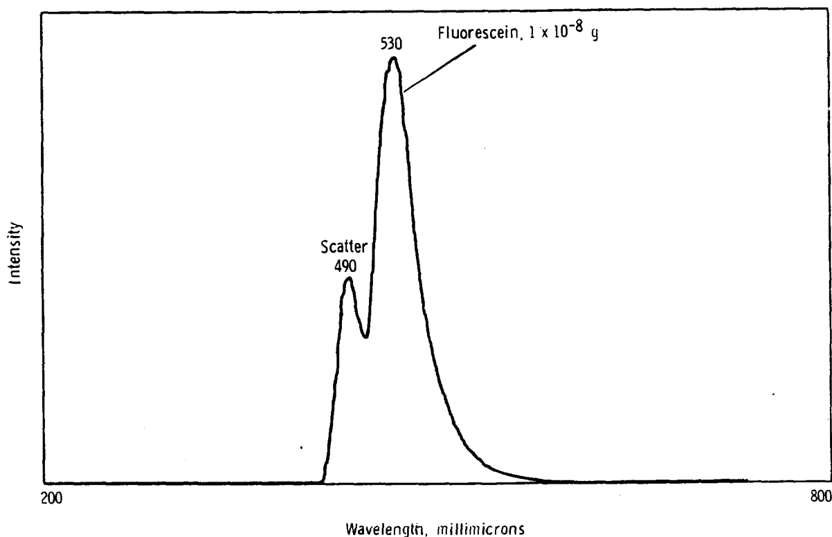
FIGURE 3.24 Fluorescein Emission
