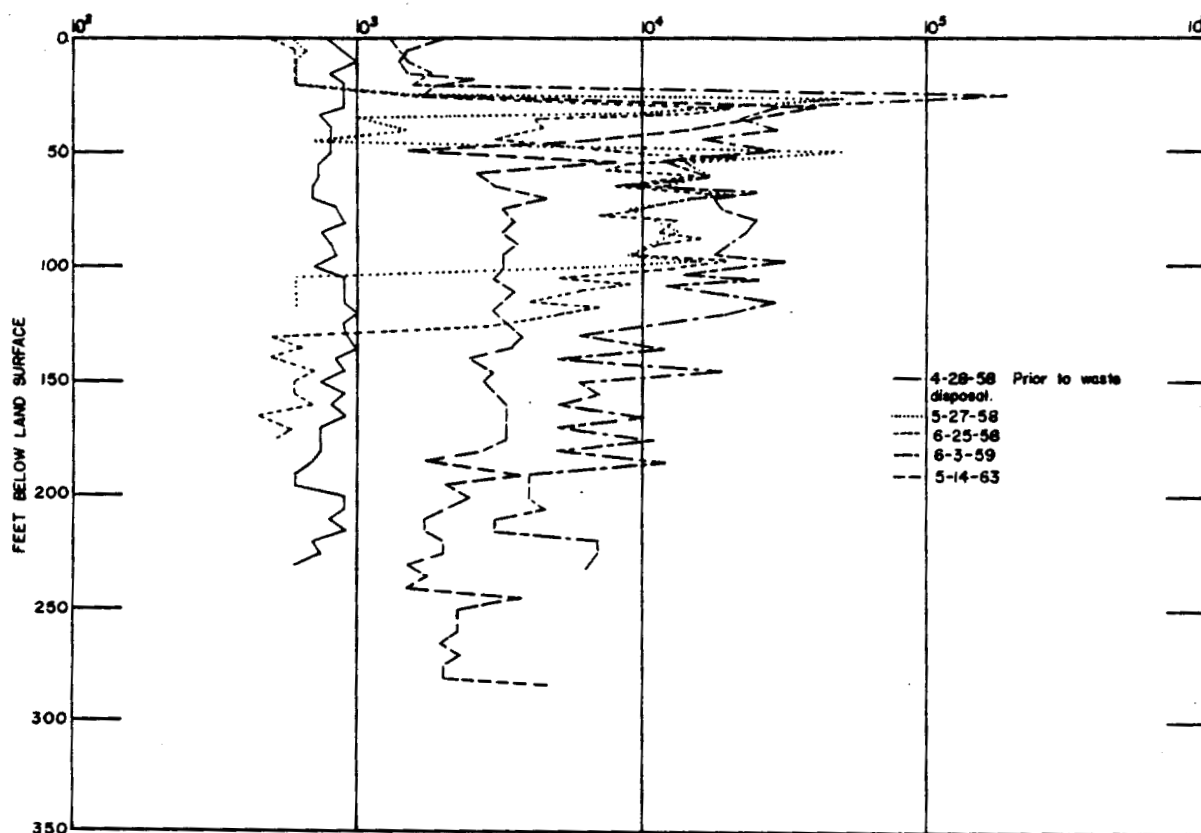
FIGURE 4.18 Probe Results in Well 299-E26-5
