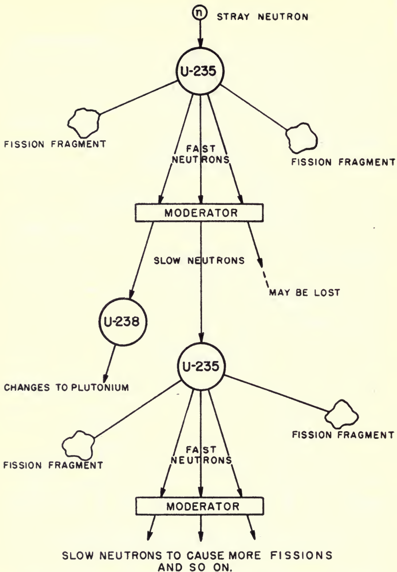
SCHEMATIC DIAGRAM OF FISSION CHAIN REACTION USING A MODERATOR TO SLOW NEUTRONS TO SPEEDS MORE LIKELY TO CAUSE FISSION
