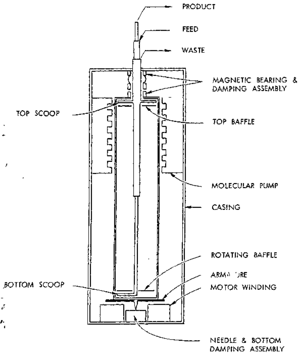
Figure 1 SCHEMATIC REPRESENTATION OF TYPICAL ZIPPE CENTRIFUGE
