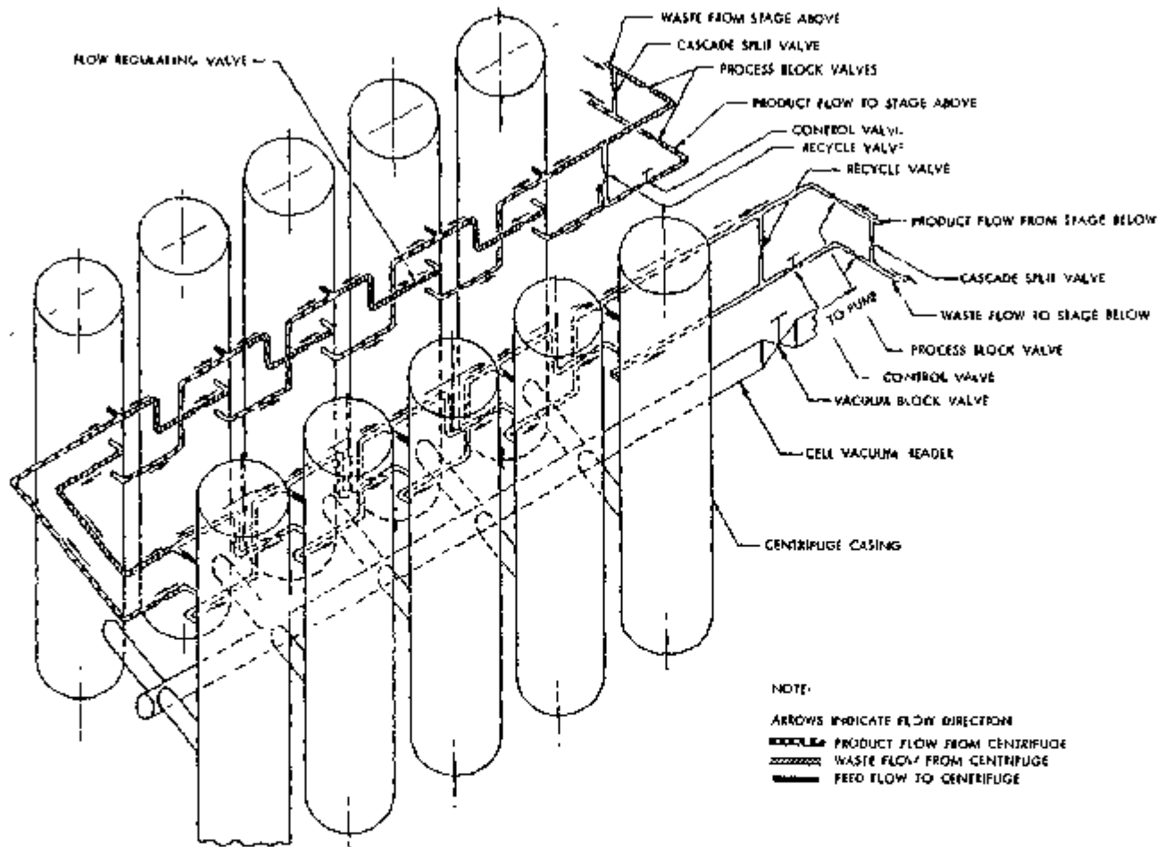
Figure 6. 10-CENTRIFUGE SERIES CELL (ONE CENTRIFUGE PER STAGE)
