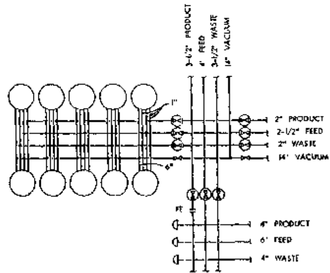
DETAIL A: TYPICAL PIPING & VALVING AT POINT WHERE THE SUB GROUP PIPING TIES INTO STAGE PIPING
