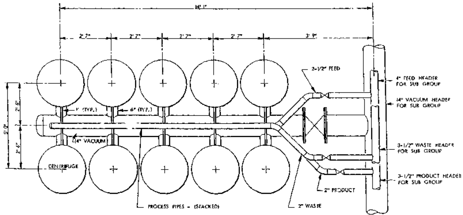
Figure 5 10-CENTRIFUGE PARALLEL CELL
