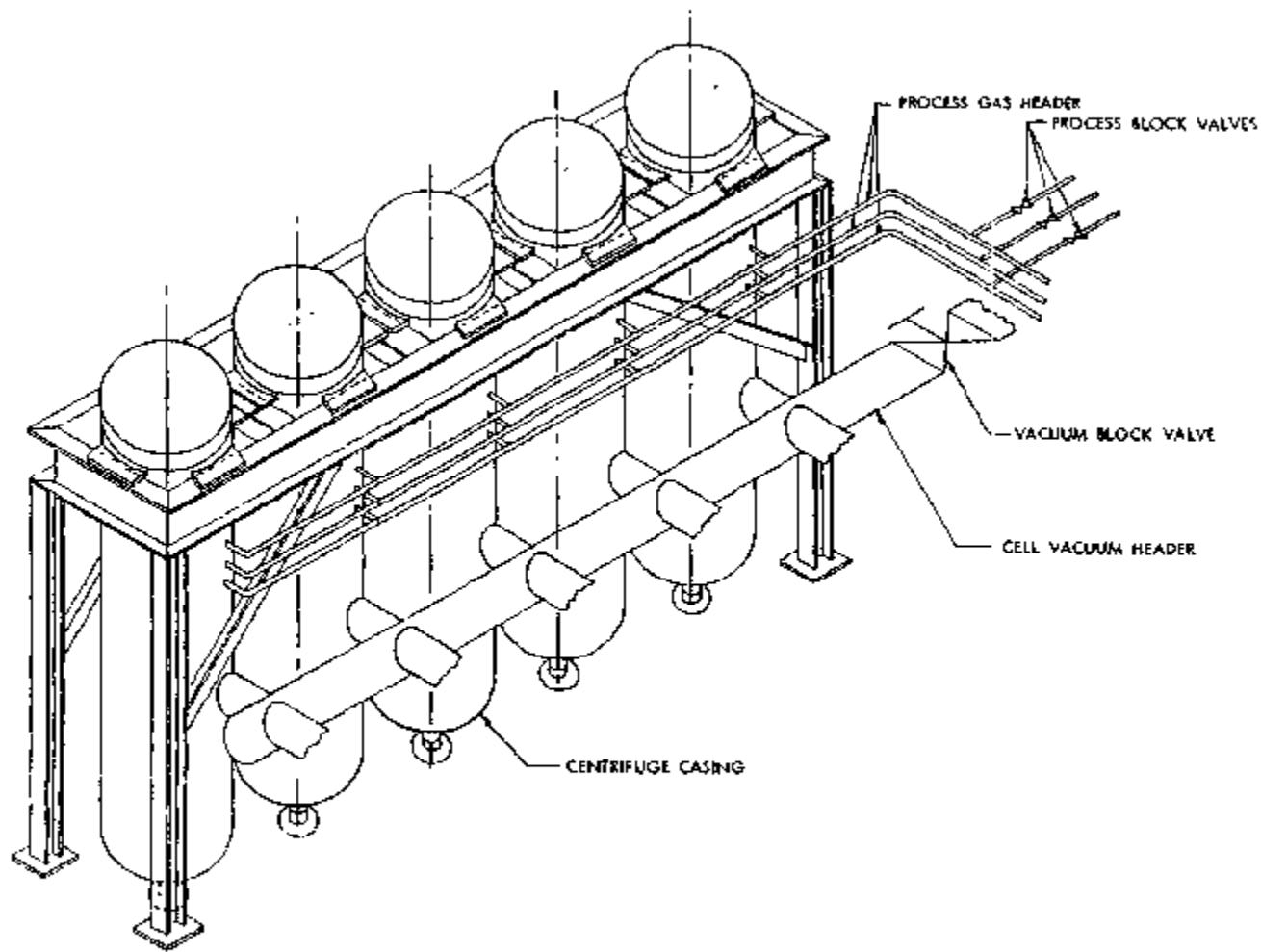
Figure 4 ONE-HALF OF A 10-CENTRIFUGE PARALLEL CELL
